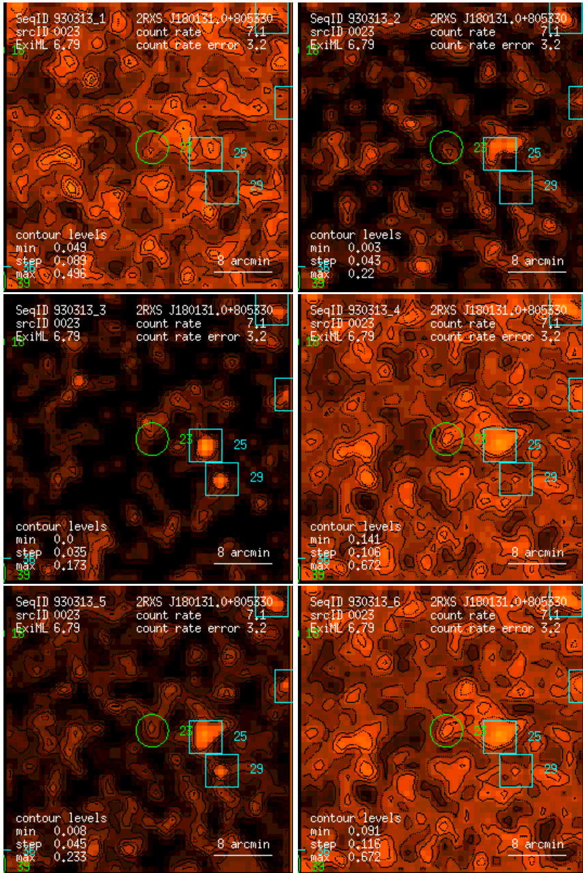
Figure 23: RASS 930313: detection 0023: band rate images, Gaussian filter: (1) PSPC channels 11 – 41, (2) 52 – 90, (3) 91 – 201, (4) 11 – 235, (5) 52 – 201, (6) 11 – 201. Broad band rates in counts/ks. Band rate contour levels in counts/ks/arcmin 2 .
