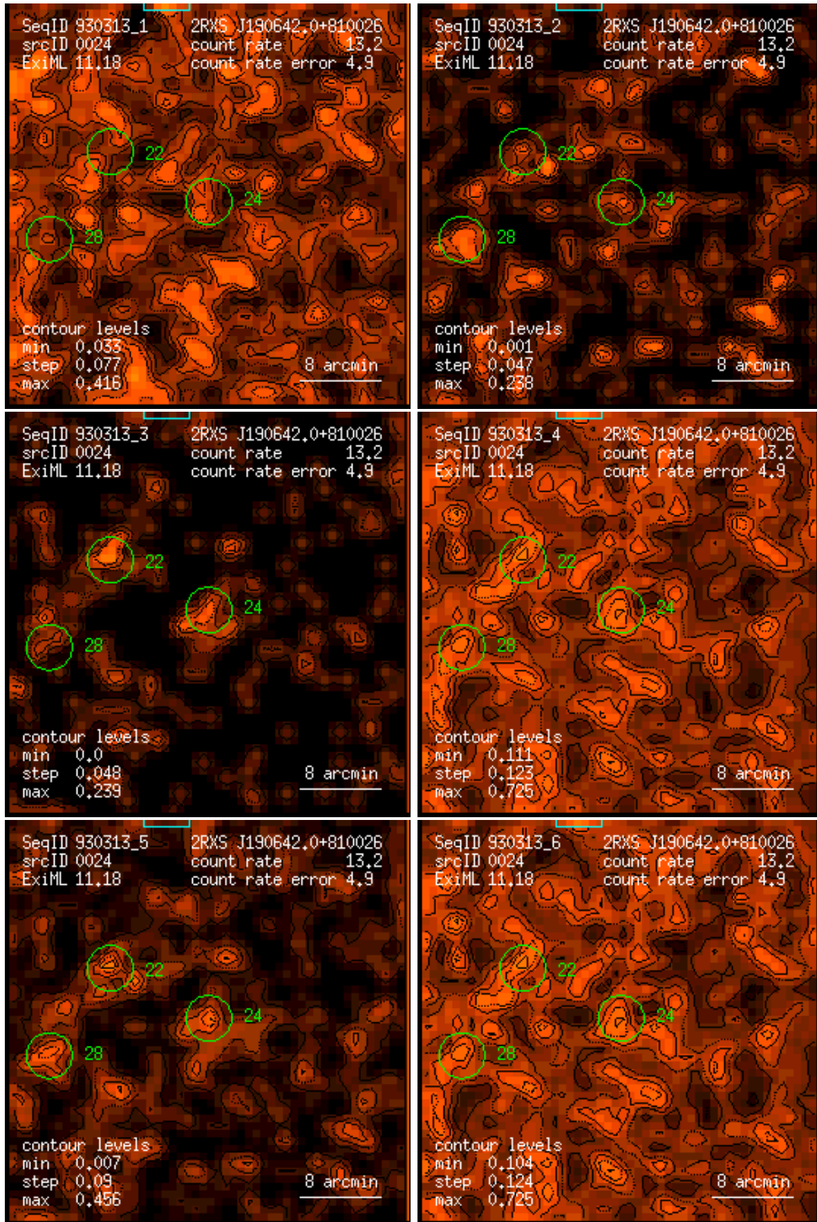
Figure 24: RASS 930313: detection 0024: band rate images, Gaussian filter: (1) PSPC channels 11 – 41, (2) 52 – 90, (3) 91 – 201, (4) 11 – 235, (5) 52 – 201, (6) 11 – 201. Broad band rates in counts/ks. Band rate contour levels in counts/ks/arcmin 2 .
