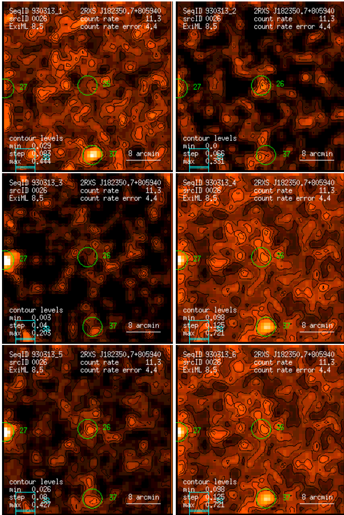
Figure 26: RASS 930313: detection 0026: band rate images, Gaussian filter: (1) PSPC channels 11 – 41, (2) 52 – 90, (3) 91 – 201, (4) 11 – 235, (5) 52 – 201, (6) 11 – 201. Broad band rates in counts/ks. Band rate contour levels in counts/ks/arcmin 2 .
