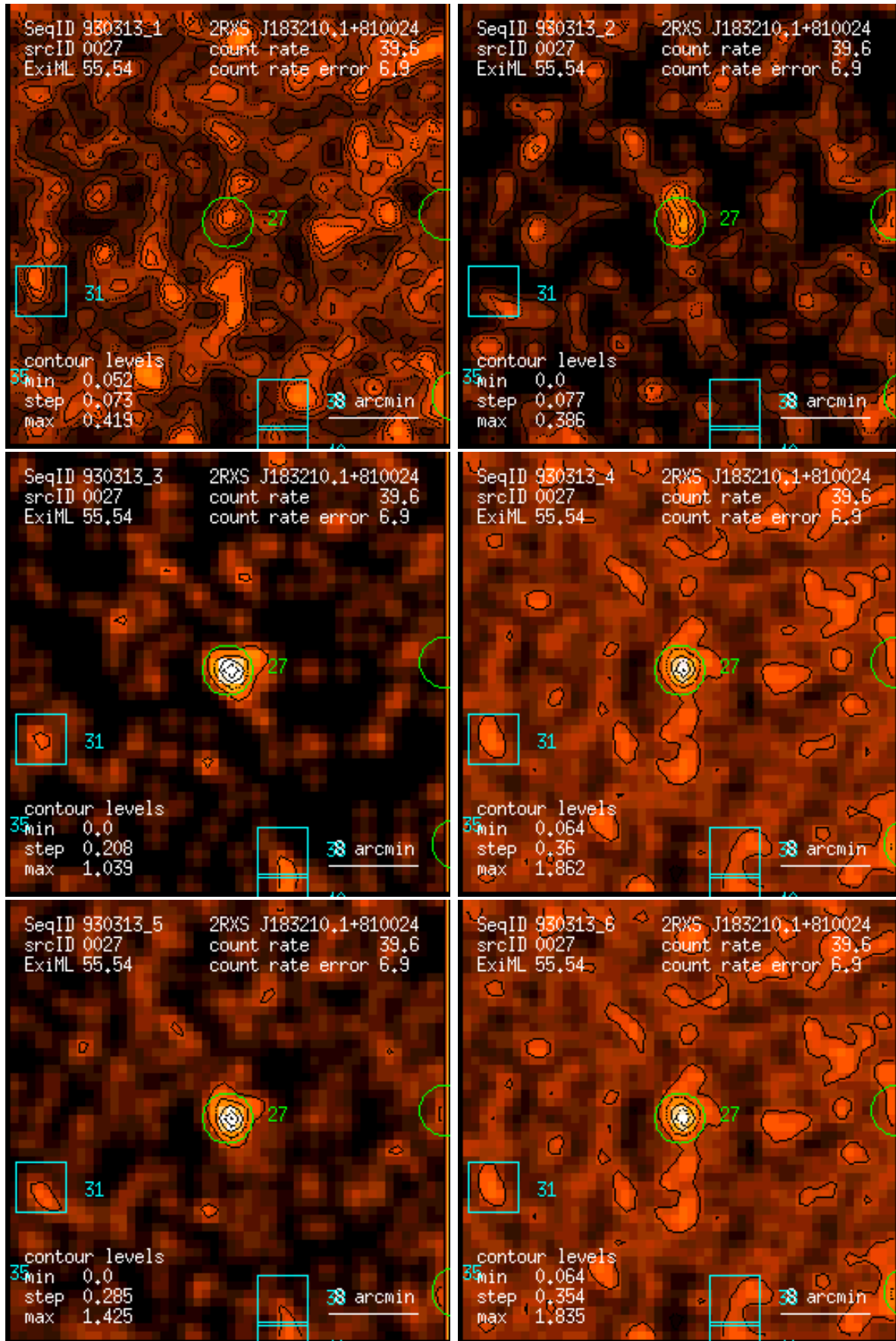
Figure 27: RASS 930313: detection 0027: band rate images, Gaussian filter: (1) PSPC channels 11 – 41, (2) 52 – 90, (3) 91 – 201, (4) 11 – 235, (5) 52 – 201, (6) 11 – 201. Broad band rates in counts/ks. Band rate contour levels in counts/ks/arcmin 2 .
