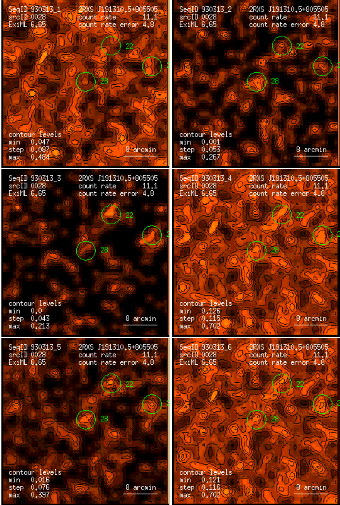
Figure 28: RASS 930313: detection 0028: band rate images, Gaussian filter: (1) PSPC channels 11 – 41, (2) 52 – 90, (3) 91 – 201, (4) 11 – 235, (5) 52 – 201, (6) 11 – 201. Broad band rates in counts/ks. Band rate contour levels in counts/ks/arcmin 2 .
