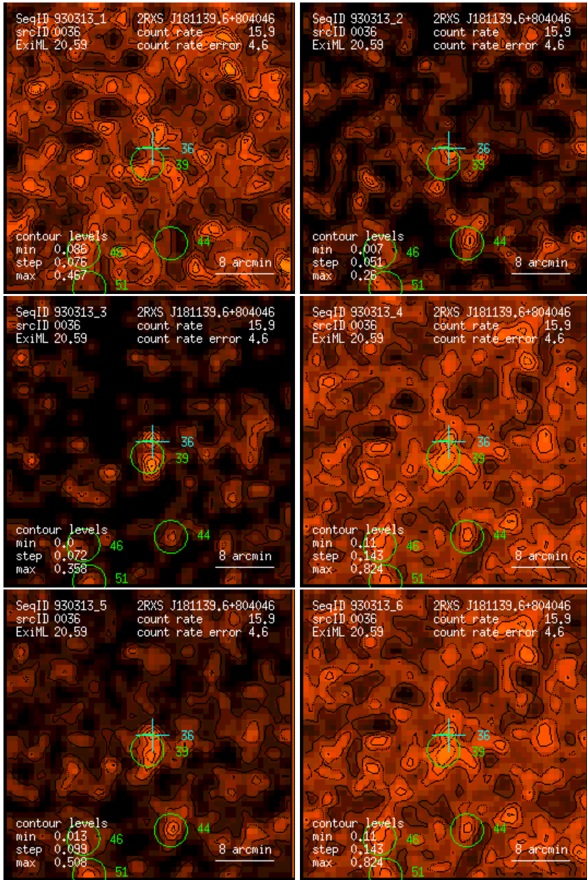
Figure 36: RASS 930313: detection 0036: band rate images, Gaussian filter: (1) PSPC channels 11 – 41, (2) 52 – 90, (3) 91 – 201, (4) 11 – 235, (5) 52 – 201, (6) 11 – 201. Broad band rates in counts/ks. Band rate contour levels in counts/ks/arcmin 2 .
