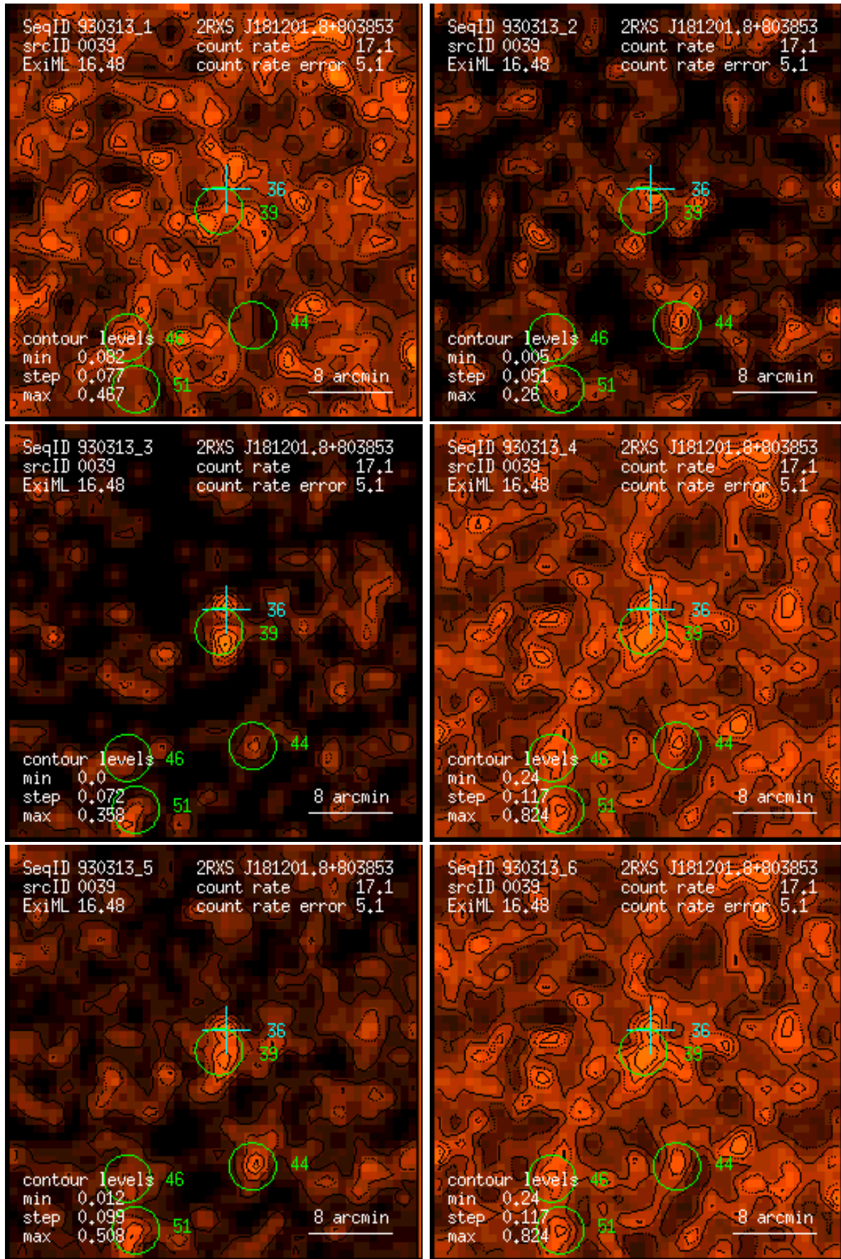
Figure 39: RASS 930313: detection 0039: band rate images, Gaussian filter: (1) PSPC channels 11 – 41, (2) 52 – 90, (3) 91 – 201, (4) 11 – 235, (5) 52 – 201, (6) 11 – 201. Broad band rates in counts/ks. Band rate contour levels in counts/ks/arcmin 2 .
