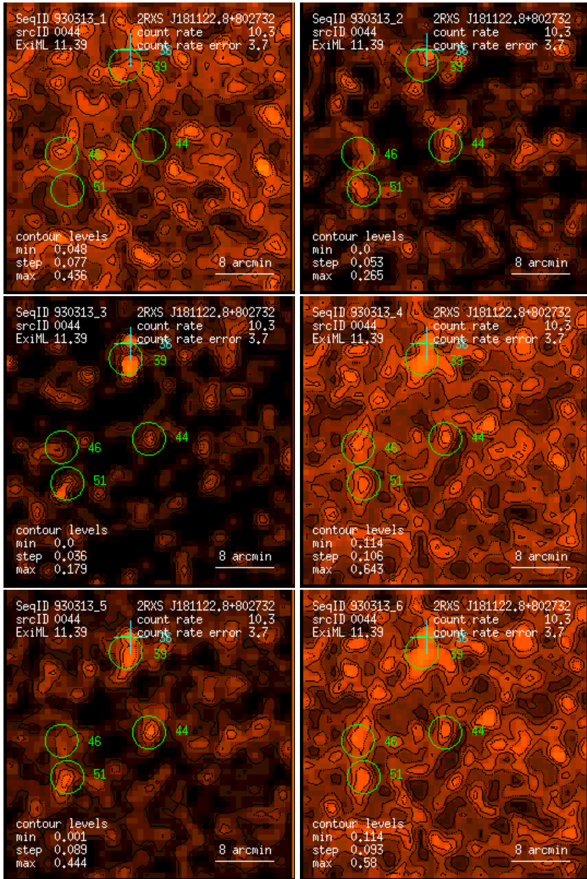
Figure 44: RASS 930313: detection 0044: band rate images, Gaussian filter: (1) PSPC channels 11 – 41, (2) 52 – 90, (3) 91 – 201, (4) 11 – 235, (5) 52 – 201, (6) 11 – 201. Broad band rates in counts/ks. Band rate contour levels in counts/ks/arcmin 2 .
