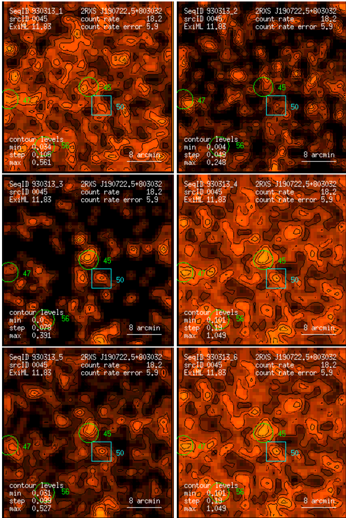
Figure 45: RASS 930313: detection 0045: band rate images, Gaussian filter: (1) PSPC channels 11 – 41, (2) 52 – 90, (3) 91 – 201, (4) 11 – 235, (5) 52 – 201, (6) 11 – 201. Broad band rates in counts/ks. Band rate contour levels in counts/ks/arcmin 2 .
