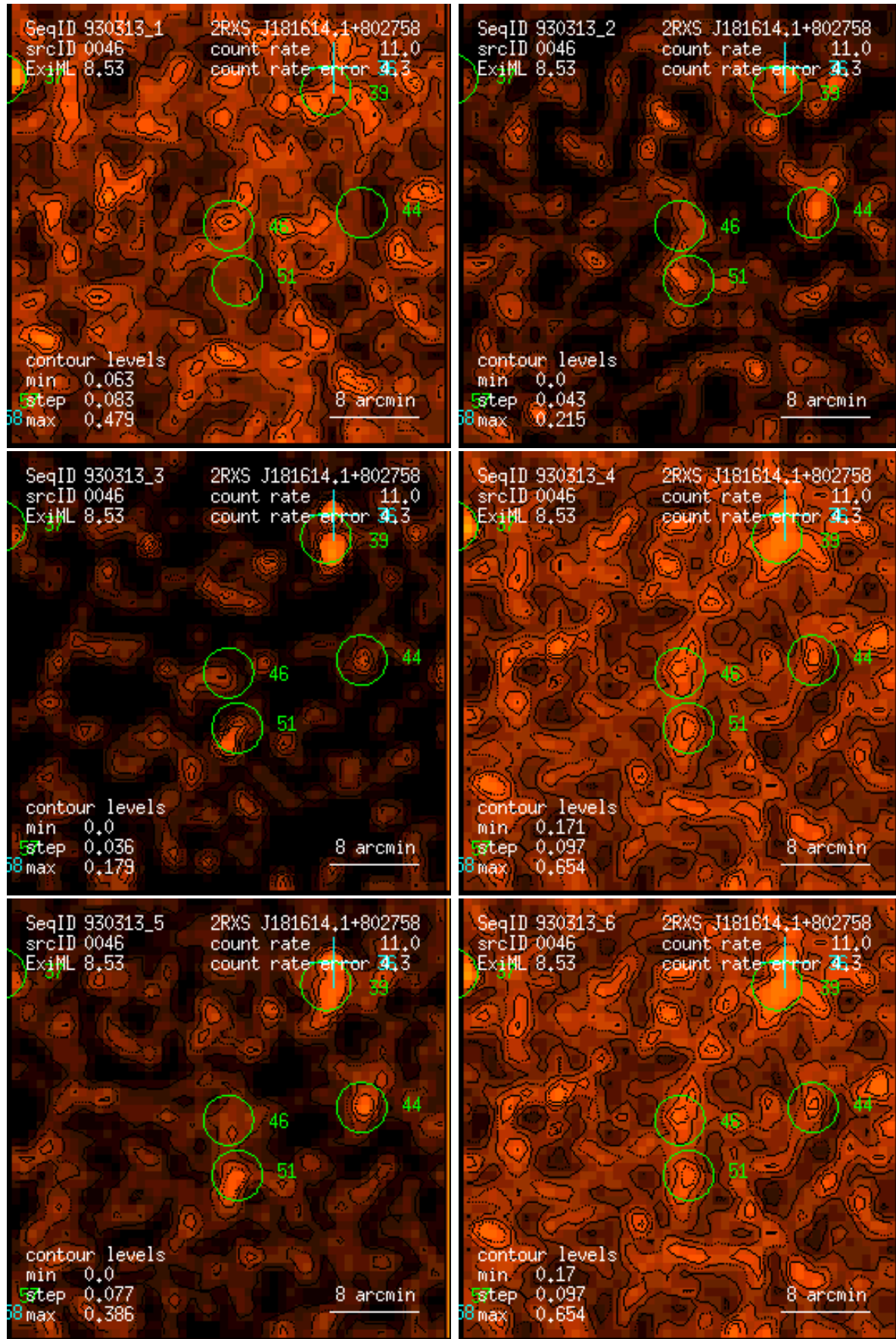
Figure 46: RASS 930313: detection 0046: band rate images, Gaussian filter: (1) PSPC channels 11 – 41, (2) 52 – 90, (3) 91 – 201, (4) 11 – 235, (5) 52 – 201, (6) 11 – 201. Broad band rates in counts/ks. Band rate contour levels in counts/ks/arcmin 2 .
