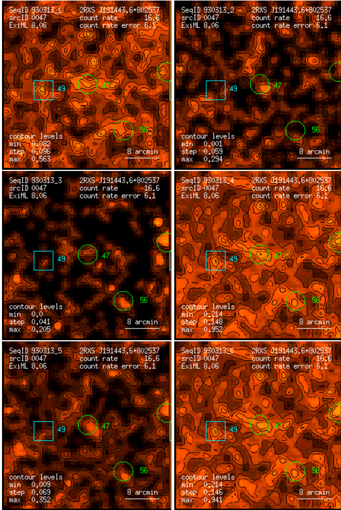
Figure 47: RASS 930313: detection 0047: band rate images, Gaussian filter: (1) PSPC channels 11 – 41, (2) 52 – 90, (3) 91 – 201, (4) 11 – 235, (5) 52 – 201, (6) 11 – 201. Broad band rates in counts/ks. Band rate contour levels in counts/ks/arcmin 2 .
