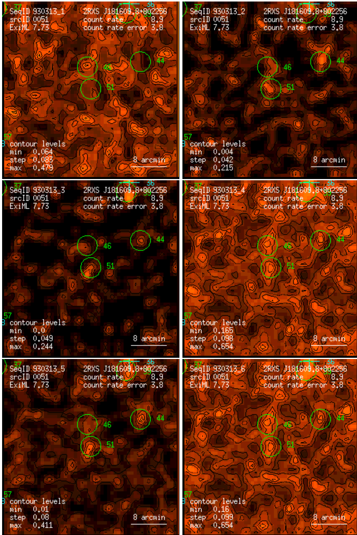
Figure 51: RASS 930313: detection 0051: band rate images, Gaussian filter: (1) PSPC channels 11 – 41, (2) 52 – 90, (3) 91 – 201, (4) 11 – 235, (5) 52 – 201, (6) 11 – 201. Broad band rates in counts/ks. Band rate contour levels in counts/ks/arcmin 2 .
