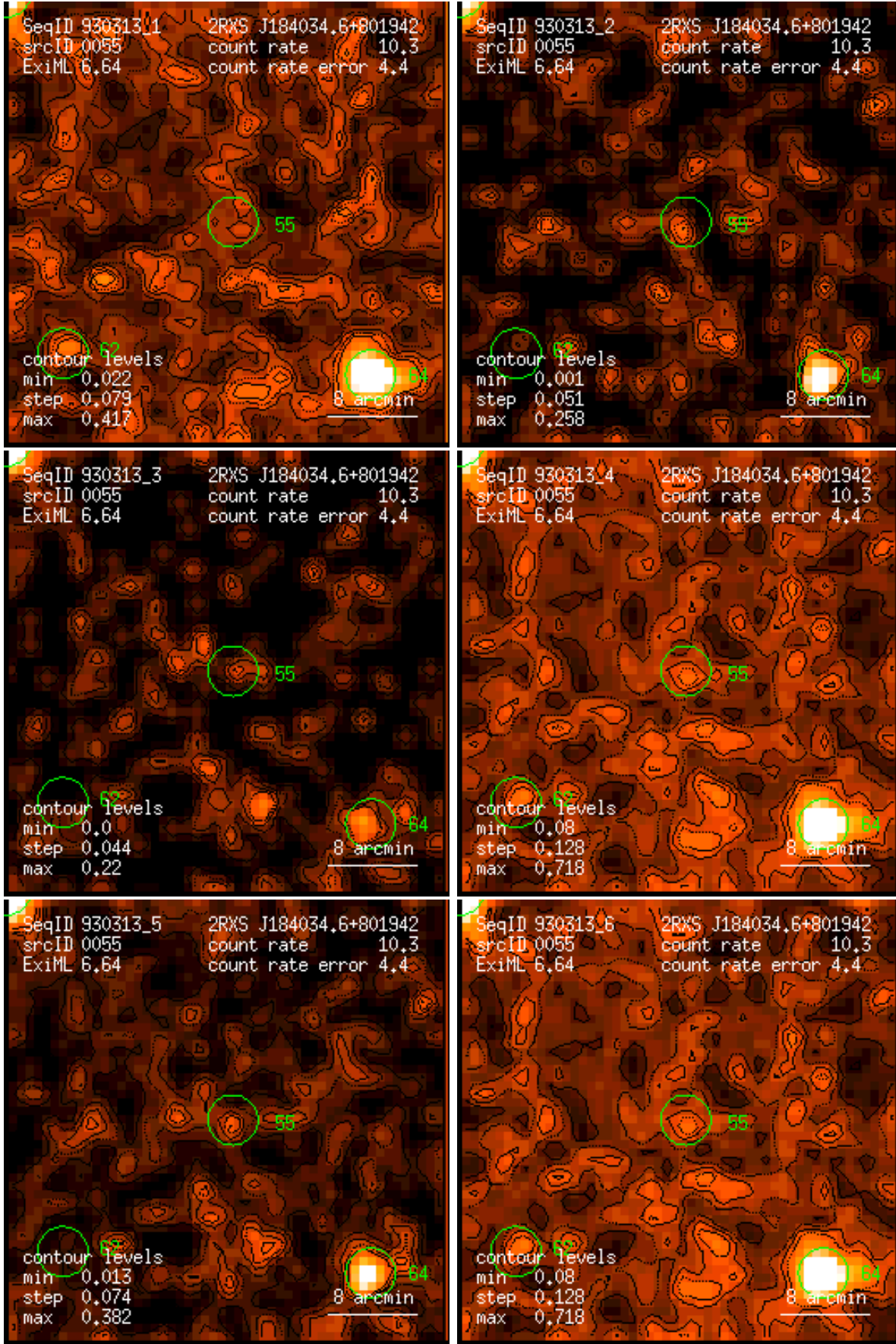
Figure 55: RASS 930313: detection 0055: band rate images, Gaussian filter: (1) PSPC channels 11 – 41, (2) 52 – 90, (3) 91 – 201, (4) 11 – 235, (5) 52 – 201, (6) 11 – 201. Broad band rates in counts/ks. Band rate contour levels in counts/ks/arcmin 2 .
