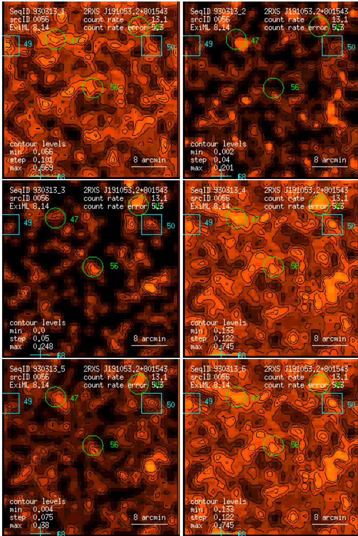
Figure 56: RASS 930313: detection 0056: band rate images, Gaussian filter: (1) PSPC channels 11 – 41, (2) 52 – 90, (3) 91 – 201, (4) 11 – 235, (5) 52 – 201, (6) 11 – 201. Broad band rates in counts/ks. Band rate contour levels in counts/ks/arcmin 2 .
