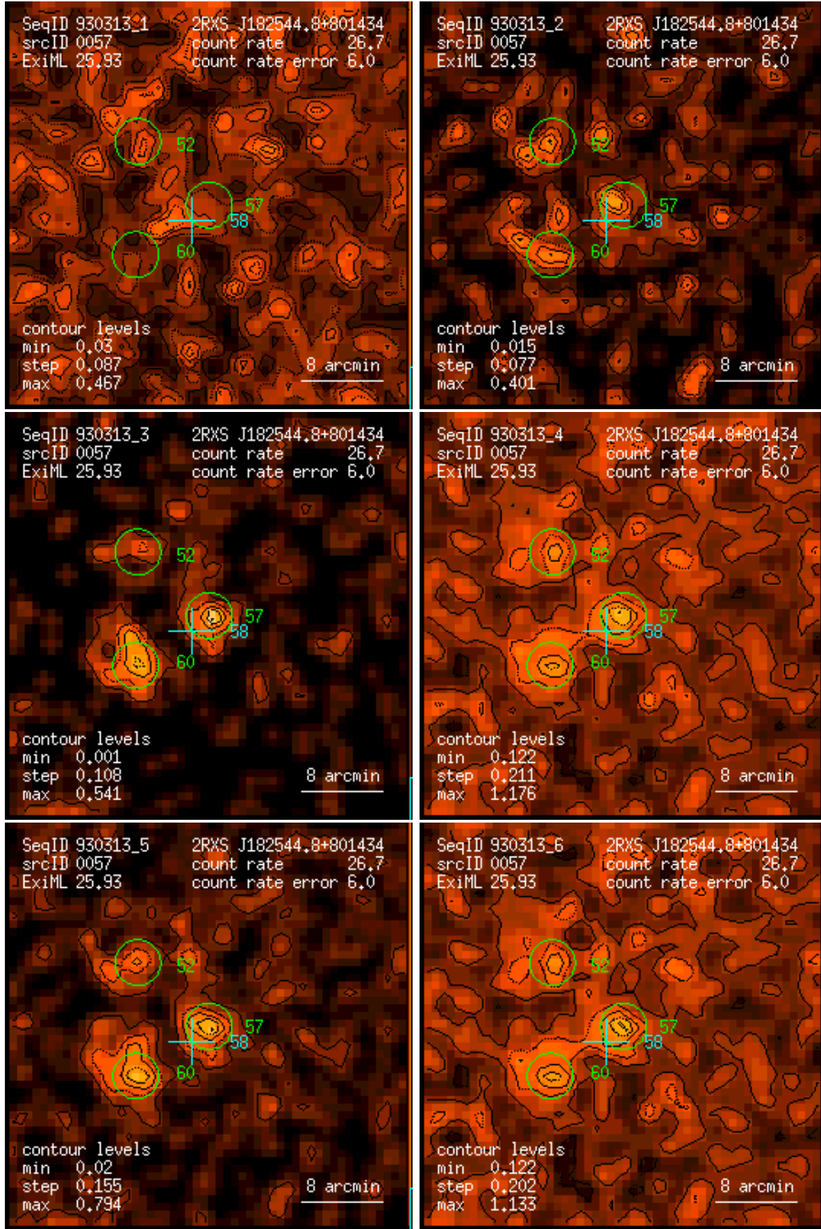
Figure 57: RASS 930313: detection 0057: band rate images, Gaussian filter: (1) PSPC channels 11 – 41, (2) 52 – 90, (3) 91 – 201, (4) 11 – 235, (5) 52 – 201, (6) 11 – 201. Broad band rates in counts/ks. Band rate contour levels in counts/ks/arcmin 2 .
