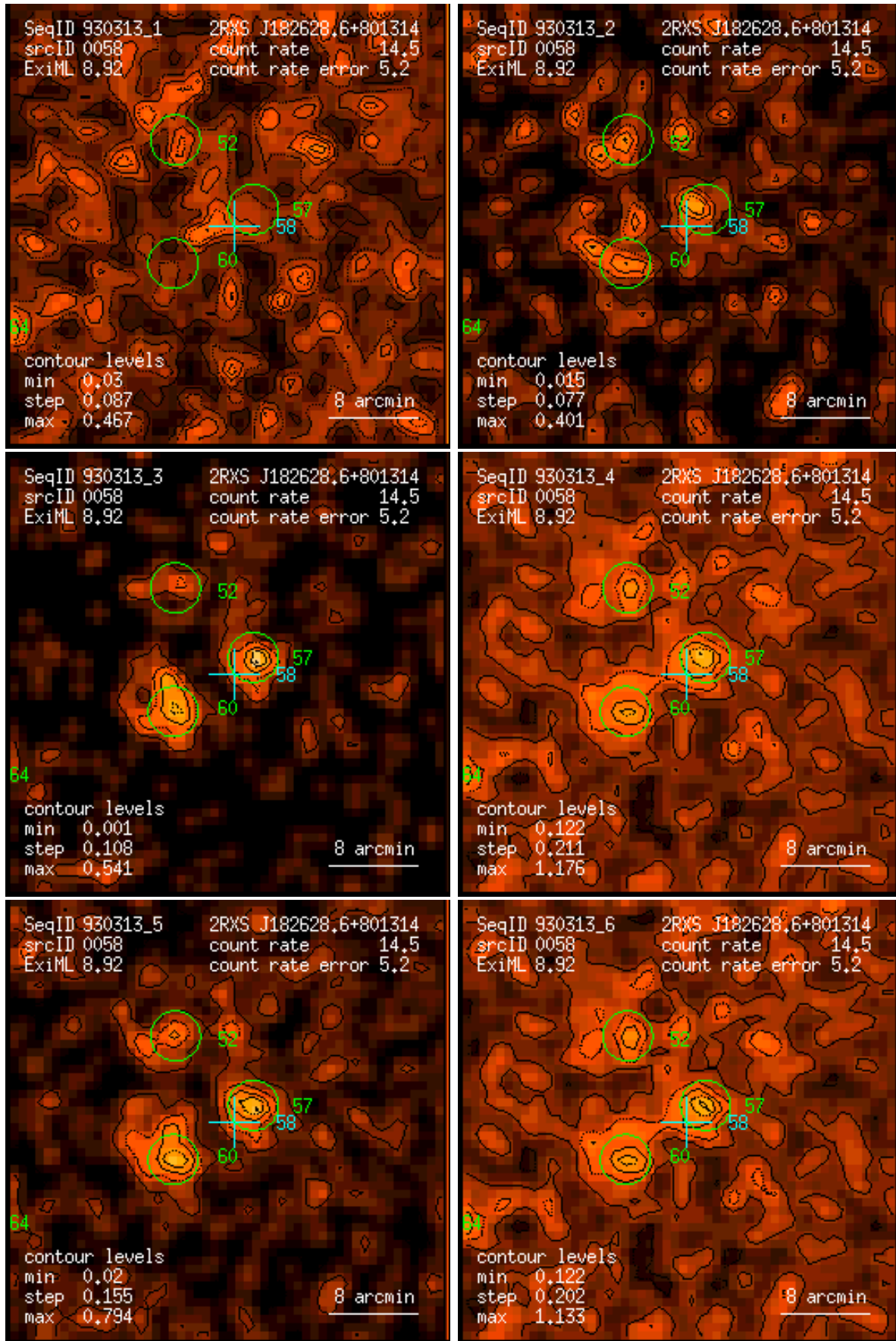
Figure 58: RASS 930313: detection 0058: band rate images, Gaussian filter: (1) PSPC channels 11 – 41, (2) 52 – 90, (3) 91 – 201, (4) 11 – 235, (5) 52 – 201, (6) 11 – 201. Broad band rates in counts/ks. Band rate contour levels in counts/ks/arcmin 2 .
