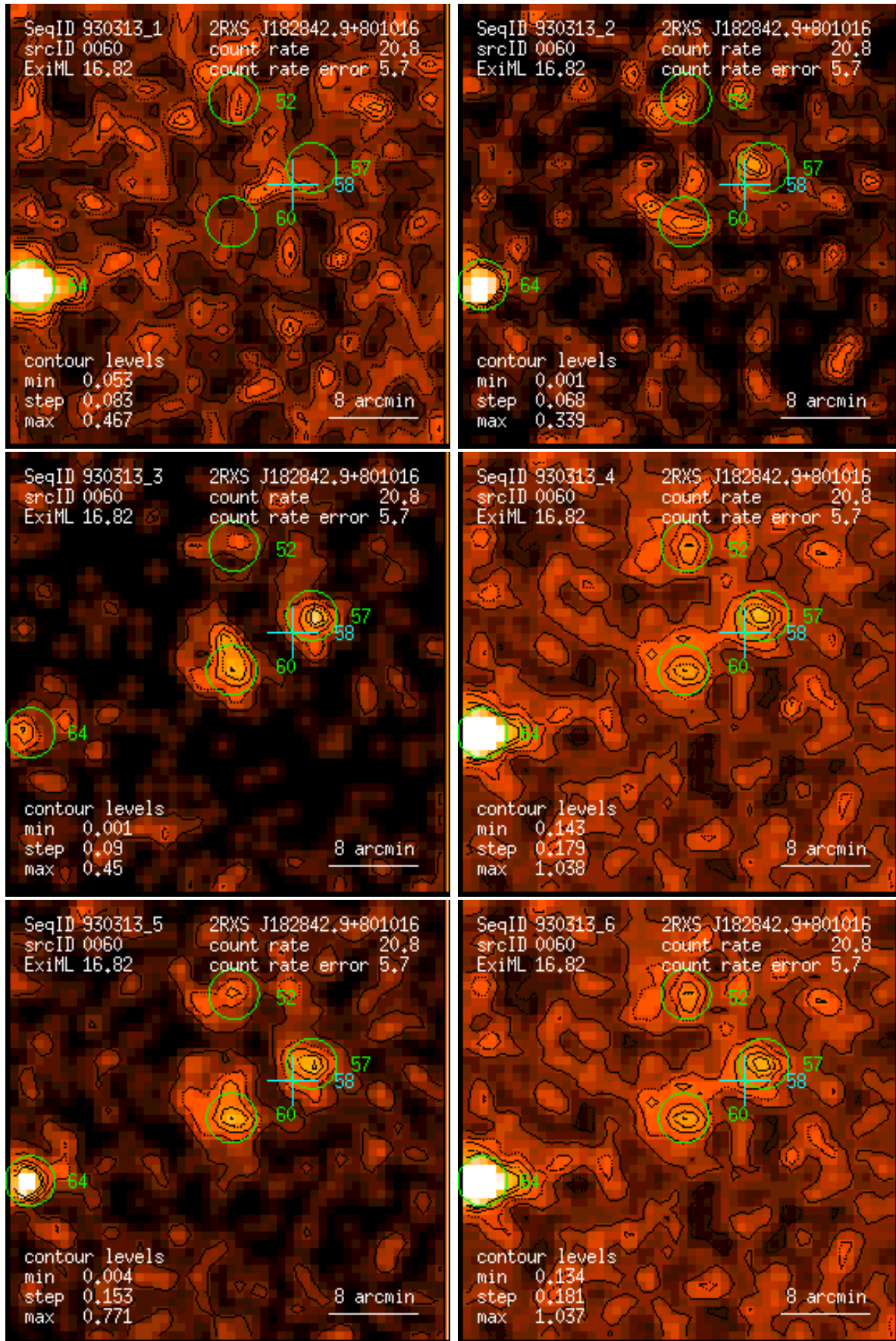
Figure 60: RASS 930313: detection 0060: band rate images, Gaussian filter: (1) PSPC channels 11 – 41, (2) 52 – 90, (3) 91 – 201, (4) 11 – 235, (5) 52 – 201, (6) 11 – 201. Broad band rates in counts/ks. Band rate contour levels in counts/ks/arcmin 2 .
