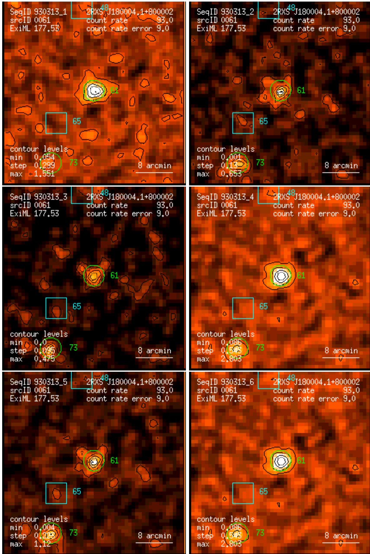
Figure 61: RASS 930313: detection 0061: band rate images, Gaussian filter: (1) PSPC channels 11 – 41, (2) 52 – 90, (3) 91 – 201, (4) 11 – 235, (5) 52 – 201, (6) 11 – 201. Broad band rates in counts/ks. Band rate contour levels in counts/ks/arcmin 2 .
