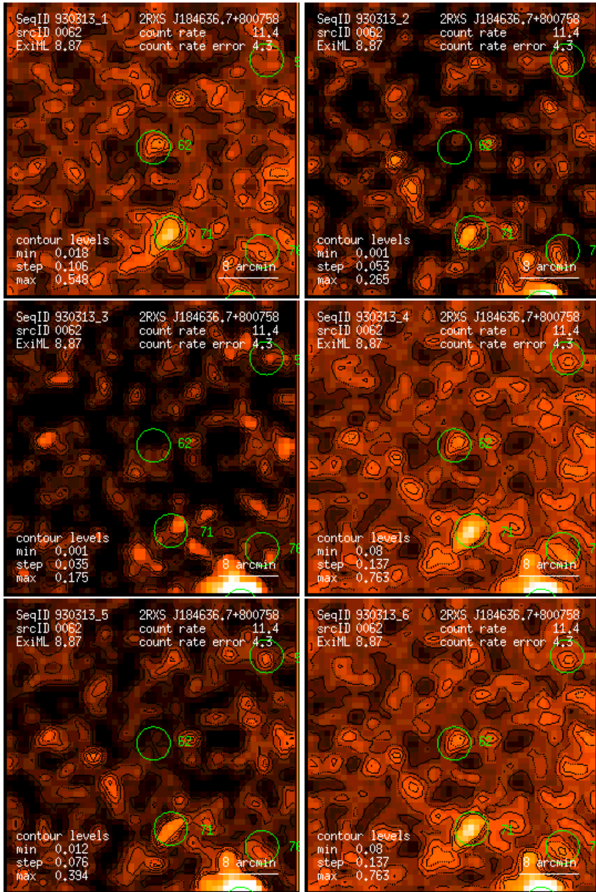
Figure 62: RASS 930313: detection 0062: band rate images, Gaussian filter: (1) PSPC channels 11 – 41, (2) 52 – 90, (3) 91 – 201, (4) 11 – 235, (5) 52 – 201, (6) 11 – 201. Broad band rates in counts/ks. Band rate contour levels in counts/ks/arcmin 2 .
