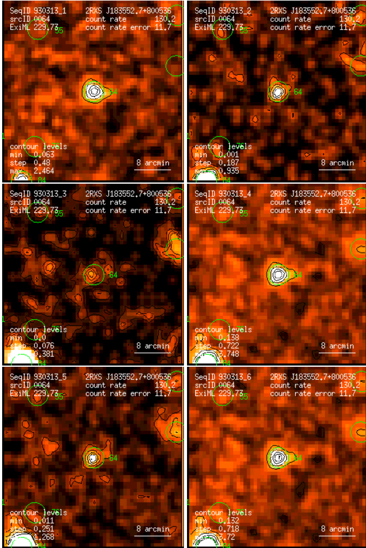
Figure 64: RASS 930313: detection 0064: band rate images, Gaussian filter: (1) PSPC channels 11 – 41, (2) 52 – 90, (3) 91 – 201, (4) 11 – 235, (5) 52 – 201, (6) 11 – 201. Broad band rates in counts/ks. Band rate contour levels in counts/ks/arcmin 2 .
