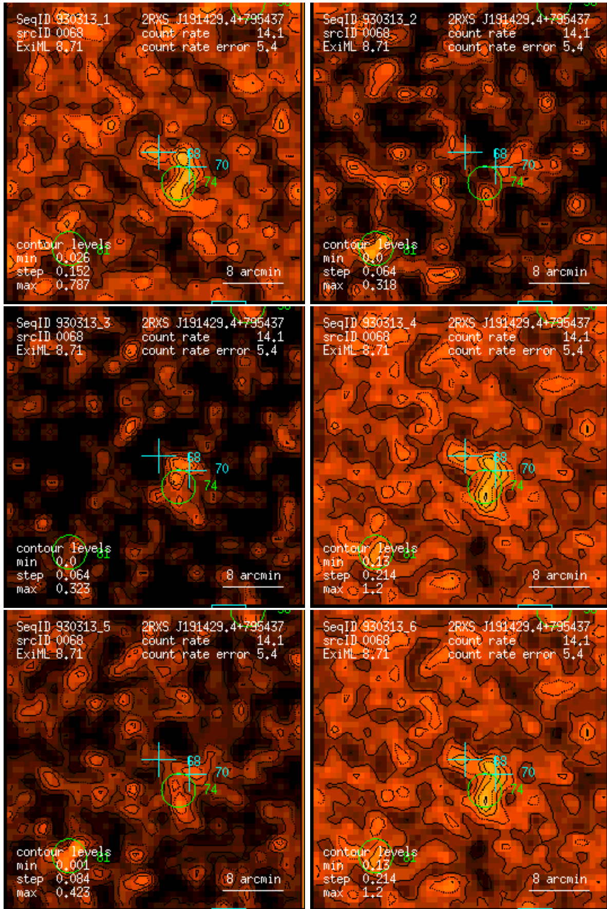
Figure 68: RASS 930313: detection 0068: band rate images, Gaussian filter: (1) PSPC channels 11 – 41, (2) 52 – 90, (3) 91 – 201, (4) 11 – 235, (5) 52 – 201, (6) 11 – 201. Broad band rates in counts/ks. Band rate contour levels in counts/ks/arcmin 2 .
