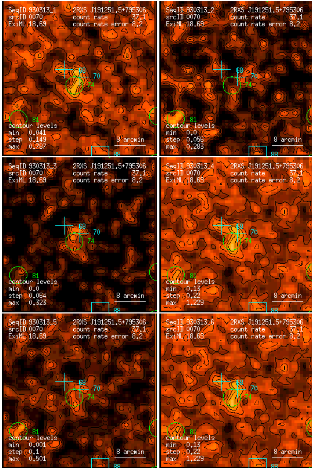
Figure 70: RASS 930313: detection 0070: band rate images, Gaussian filter: (1) PSPC channels 11 – 41, (2) 52 – 90, (3) 91 – 201, (4) 11 – 235, (5) 52 – 201, (6) 11 – 201. Broad band rates in counts/ks. Band rate contour levels in counts/ks/arcmin 2 .
