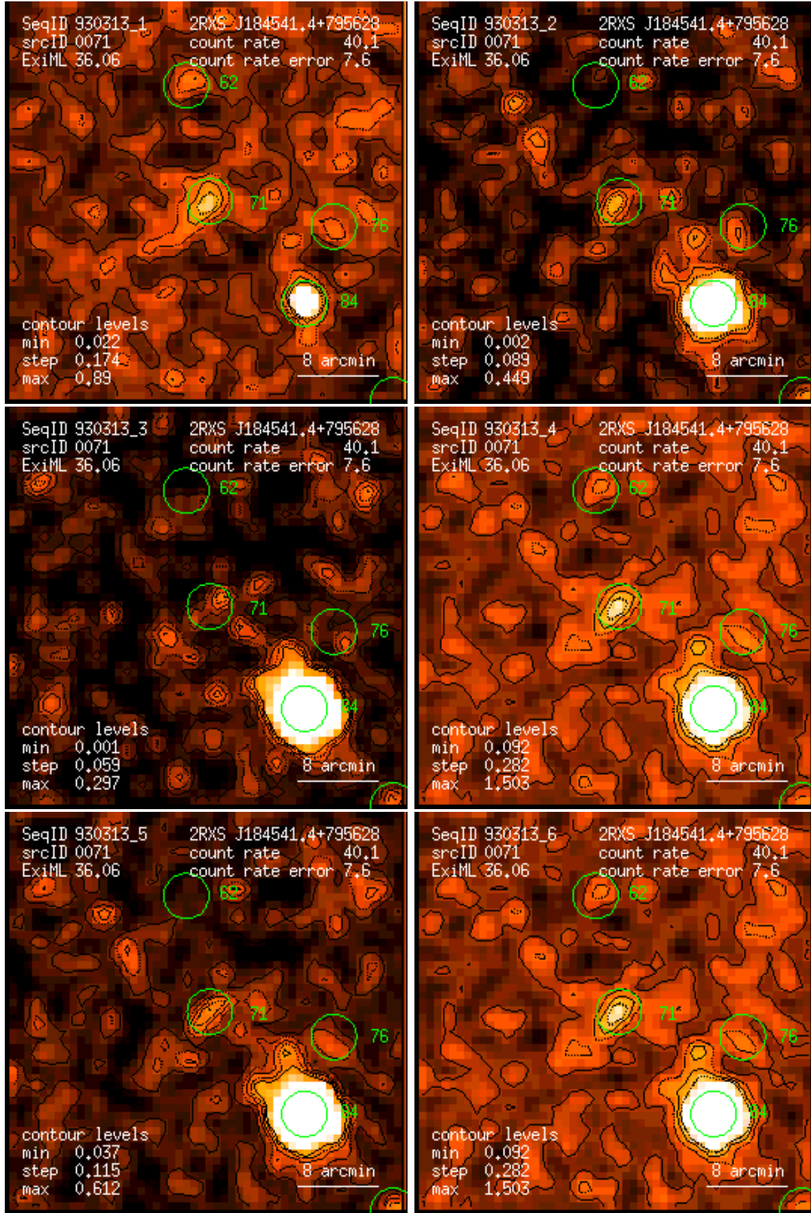
Figure 71: RASS 930313: detection 0071: band rate images, Gaussian filter: (1) PSPC channels 11 – 41, (2) 52 – 90, (3) 91 – 201, (4) 11 – 235, (5) 52 – 201, (6) 11 – 201. Broad band rates in counts/ks. Band rate contour levels in counts/ks/arcmin 2 .
