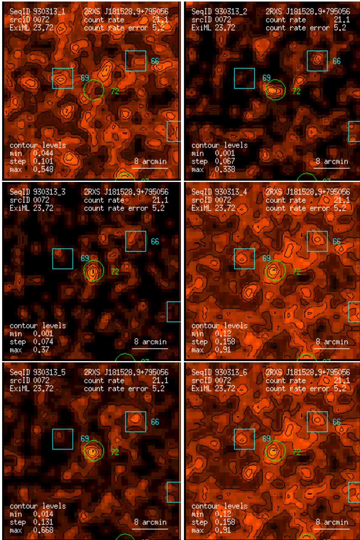
Figure 72: RASS 930313: detection 0072: band rate images, Gaussian filter: (1) PSPC channels 11 – 41, (2) 52 – 90, (3) 91 – 201, (4) 11 – 235, (5) 52 – 201, (6) 11 – 201. Broad band rates in counts/ks. Band rate contour levels in counts/ks/arcmin 2 .
