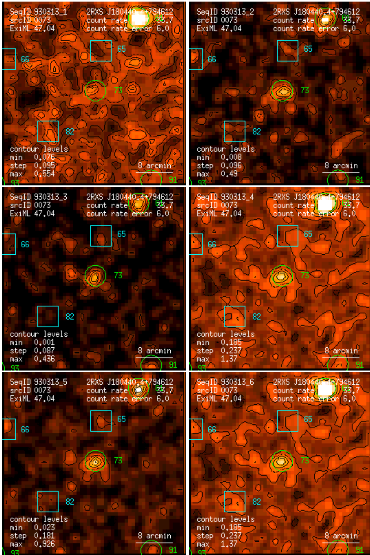
Figure 73: RASS 930313: detection 0073: band rate images, Gaussian filter: (1) PSPC channels 11 – 41, (2) 52 – 90, (3) 91 – 201, (4) 11 – 235, (5) 52 – 201, (6) 11 – 201. Broad band rates in counts/ks. Band rate contour levels in counts/ks/arcmin 2 .
