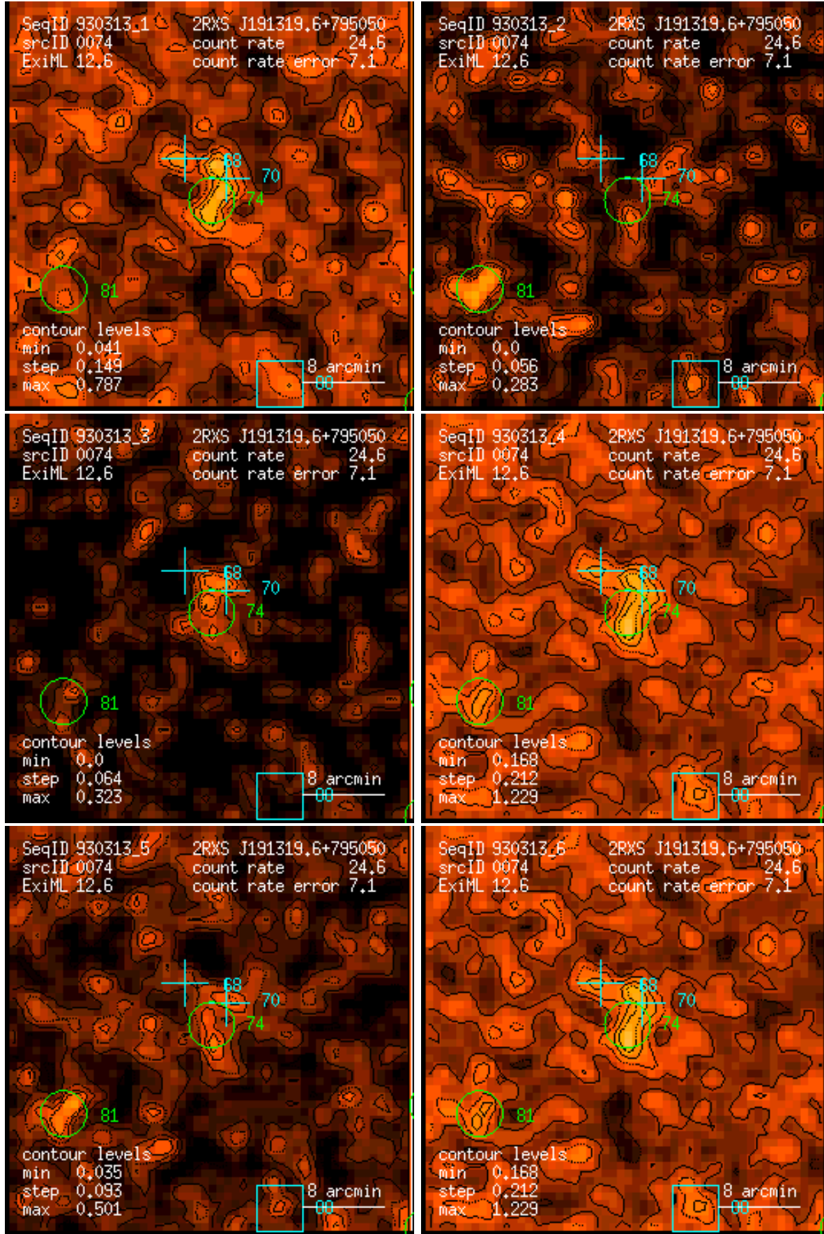
Figure 74: RASS 930313: detection 0074: band rate images, Gaussian filter: (1) PSPC channels 11 – 41, (2) 52 – 90, (3) 91 – 201, (4) 11 – 235, (5) 52 – 201, (6) 11 – 201. Broad band rates in counts/ks. Band rate contour levels in counts/ks/arcmin 2 .
