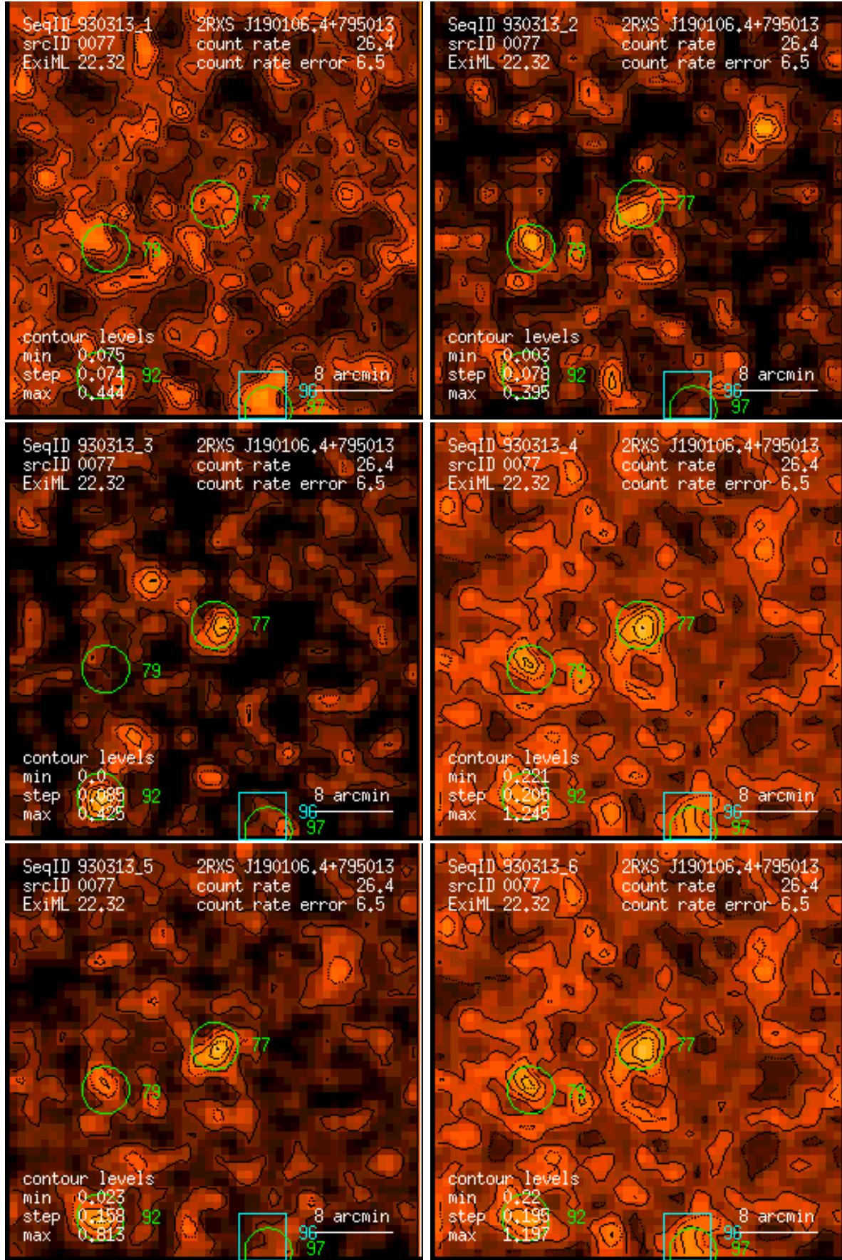
Figure 77: RASS 930313: detection 0077: band rate images, Gaussian filter: (1) PSPC channels 11 – 41, (2) 52 – 90, (3) 91 – 201, (4) 11 – 235, (5) 52 – 201, (6) 11 – 201. Broad band rates in counts/ks. Band rate contour levels in counts/ks/arcmin 2 .
