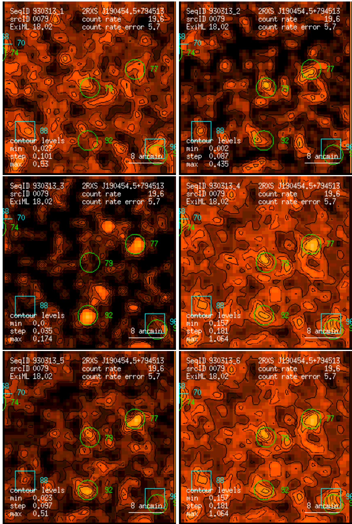
Figure 79: RASS 930313: detection 0079: band rate images, Gaussian filter: (1) PSPC channels 11 – 41, (2) 52 – 90, (3) 91 – 201, (4) 11 – 235, (5) 52 – 201, (6) 11 – 201. Broad band rates in counts/ks. Band rate contour levels in counts/ks/arcmin 2 .
