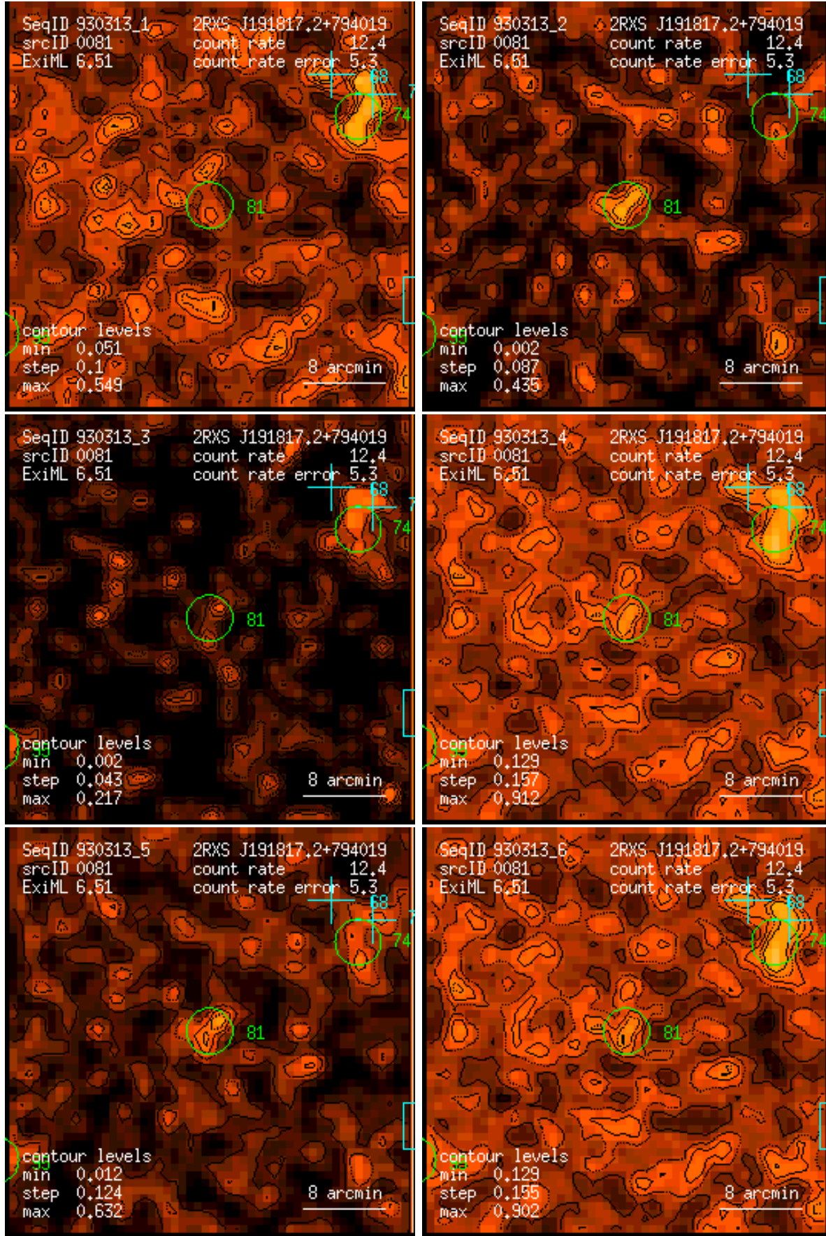
Figure 81: RASS 930313: detection 0081: band rate images, Gaussian filter: (1) PSPC channels 11 – 41, (2) 52 – 90, (3) 91 – 201, (4) 11 – 235, (5) 52 – 201, (6) 11 – 201. Broad band rates in counts/ks. Band rate contour levels in counts/ks/arcmin 2 .
