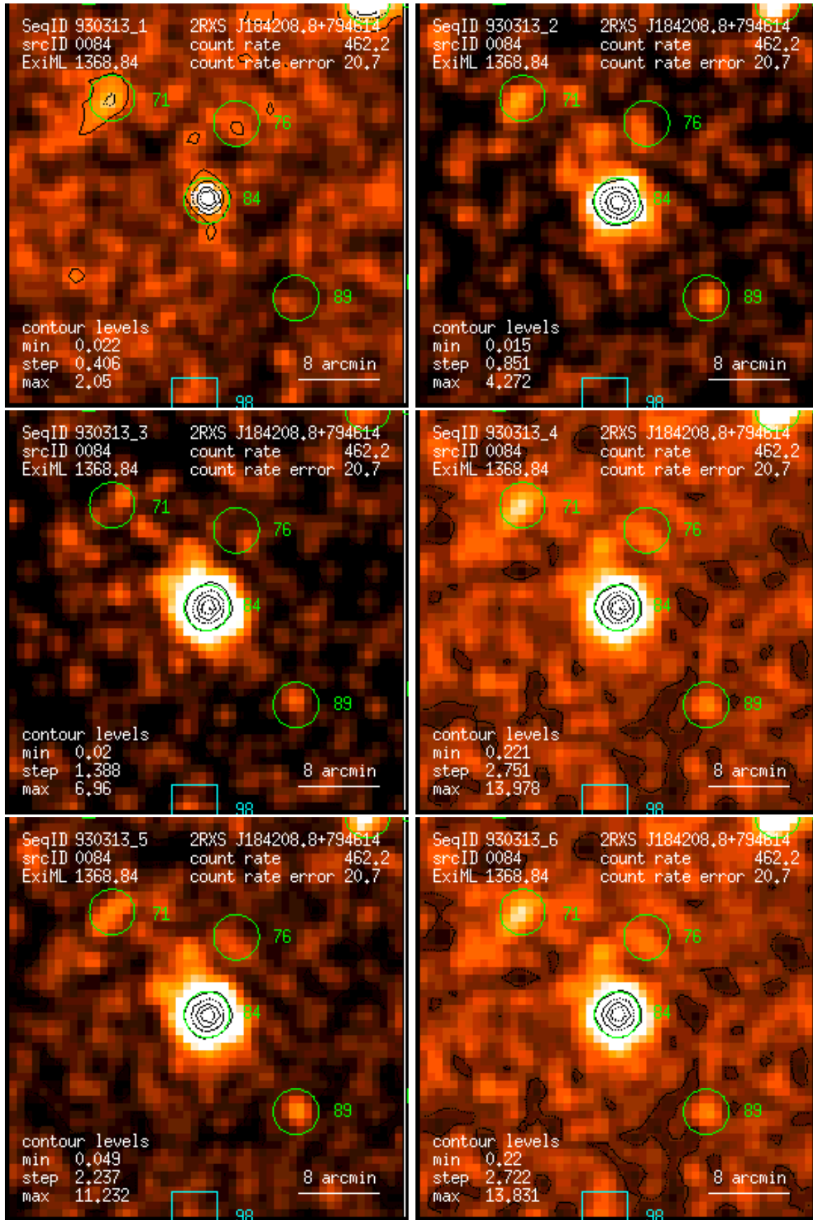
Figure 84: RASS 930313: detection 0084: band rate images, Gaussian filter: (1) PSPC channels 11 – 41, (2) 52 – 90, (3) 91 – 201, (4) 11 – 235, (5) 52 – 201, (6) 11 – 201. Broad band rates in counts/ks. Band rate contour levels in counts/ks/arcmin 2 .
