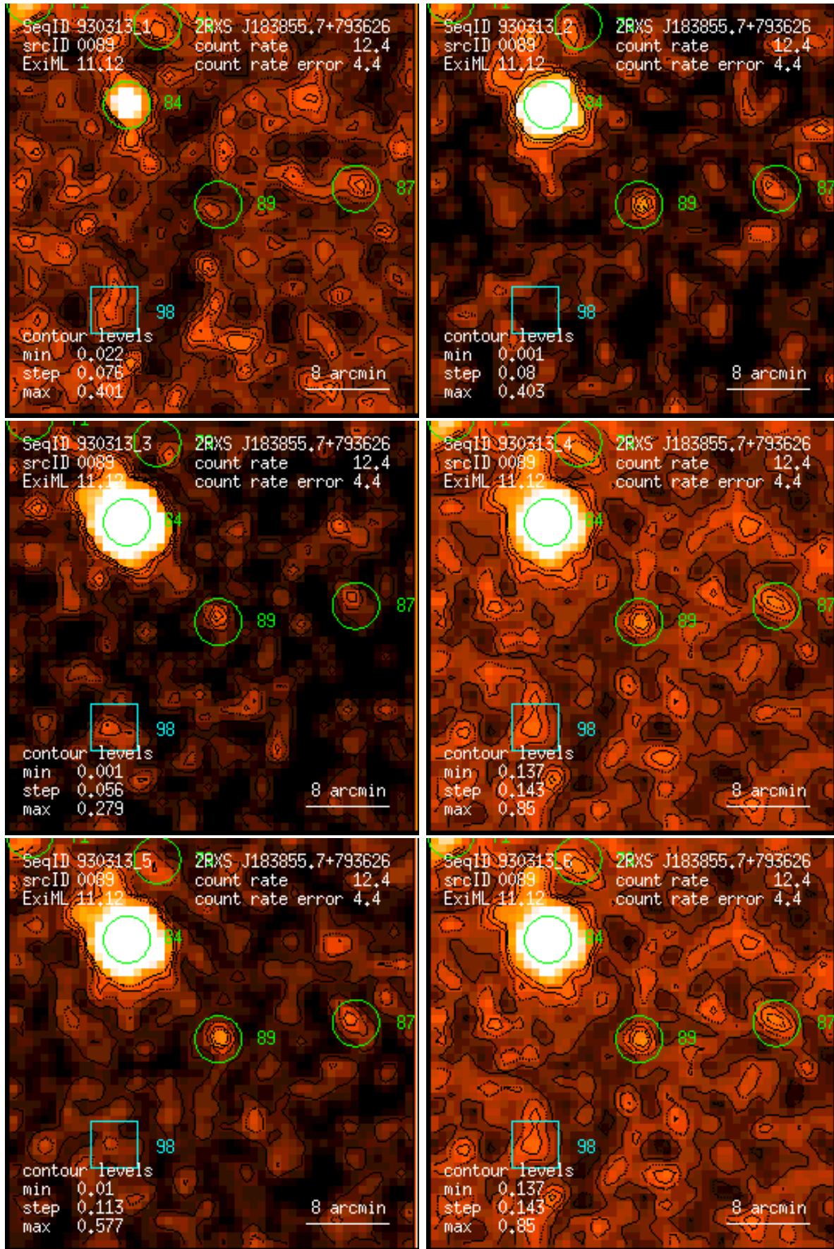
Figure 89: RASS 930313: detection 0089: band rate images, Gaussian filter: (1) PSPC channels 11 – 41, (2) 52 – 90, (3) 91 – 201, (4) 11 – 235, (5) 52 – 201, (6) 11 – 201. Broad band rates in counts/ks. Band rate contour levels in counts/ks/arcmin 2 .
