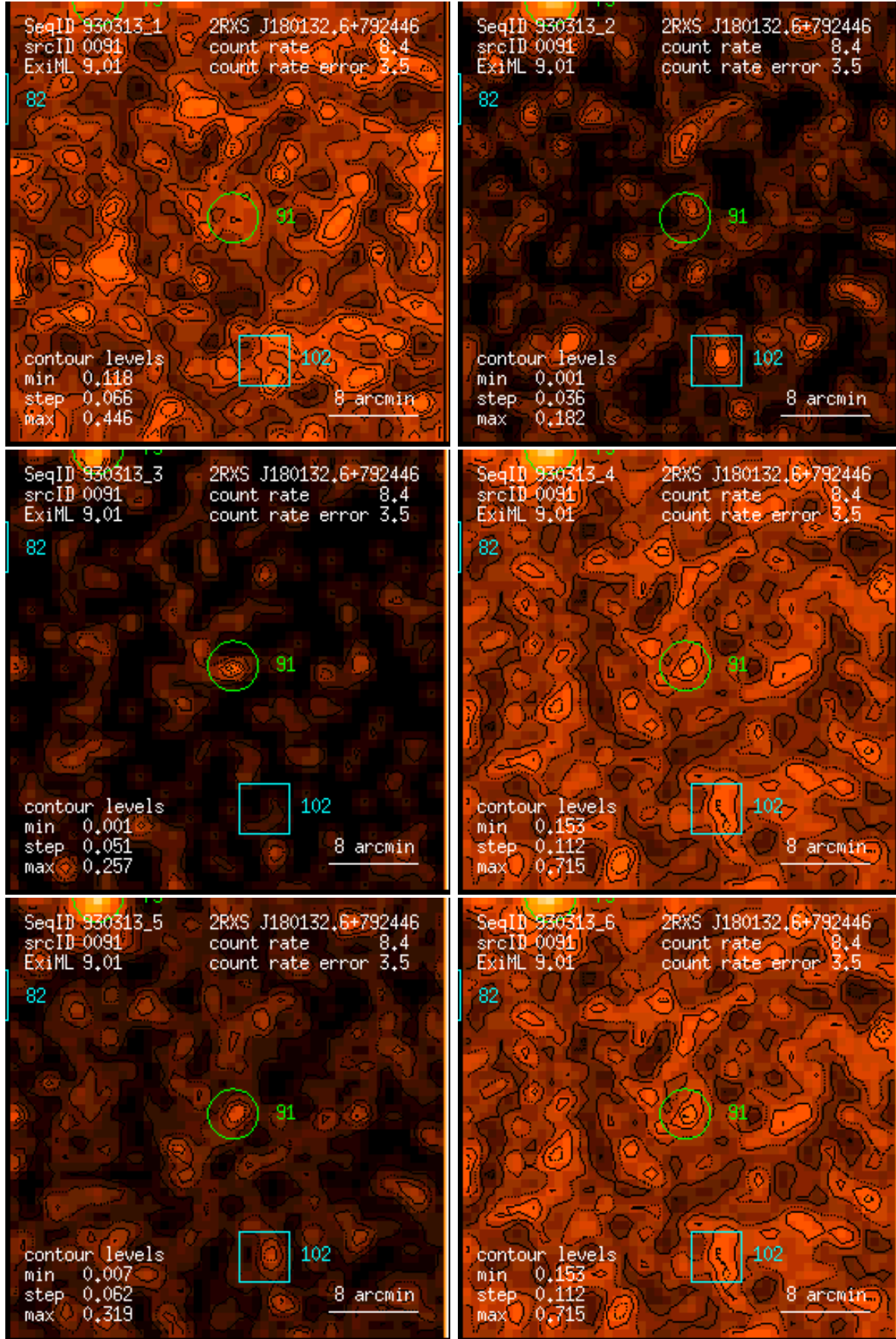
Figure 91: RASS 930313: detection 0091: band rate images, Gaussian filter: (1) PSPC channels 11 – 41, (2) 52 – 90, (3) 91 – 201, (4) 11 – 235, (5) 52 – 201, (6) 11 – 201. Broad band rates in counts/ks. Band rate contour levels in counts/ks/arcmin 2 .
