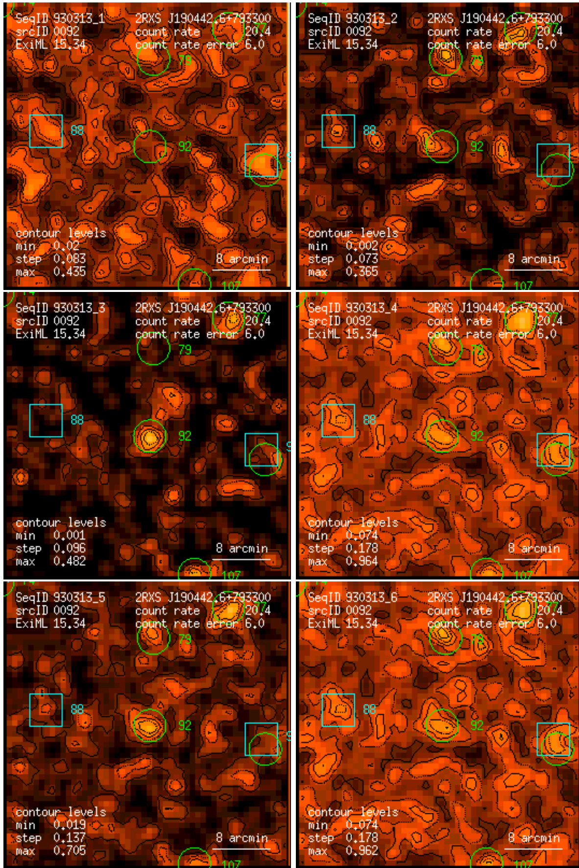
Figure 92: RASS 930313: detection 0092: band rate images, Gaussian filter: (1) PSPC channels 11 – 41, (2) 52 – 90, (3) 91 – 201, (4) 11 – 235, (5) 52 – 201, (6) 11 – 201. Broad band rates in counts/ks. Band rate contour levels in counts/ks/arcmin 2 .
