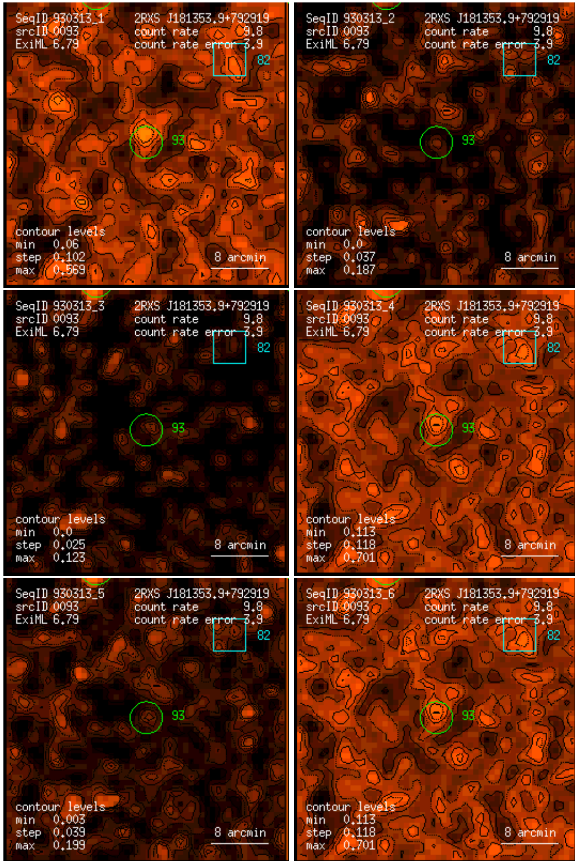
Figure 93: RASS 930313: detection 0093: band rate images, Gaussian filter: (1) PSPC channels 11 – 41, (2) 52 – 90, (3) 91 – 201, (4) 11 – 235, (5) 52 – 201, (6) 11 – 201. Broad band rates in counts/ks. Band rate contour levels in counts/ks/arcmin 2 .
