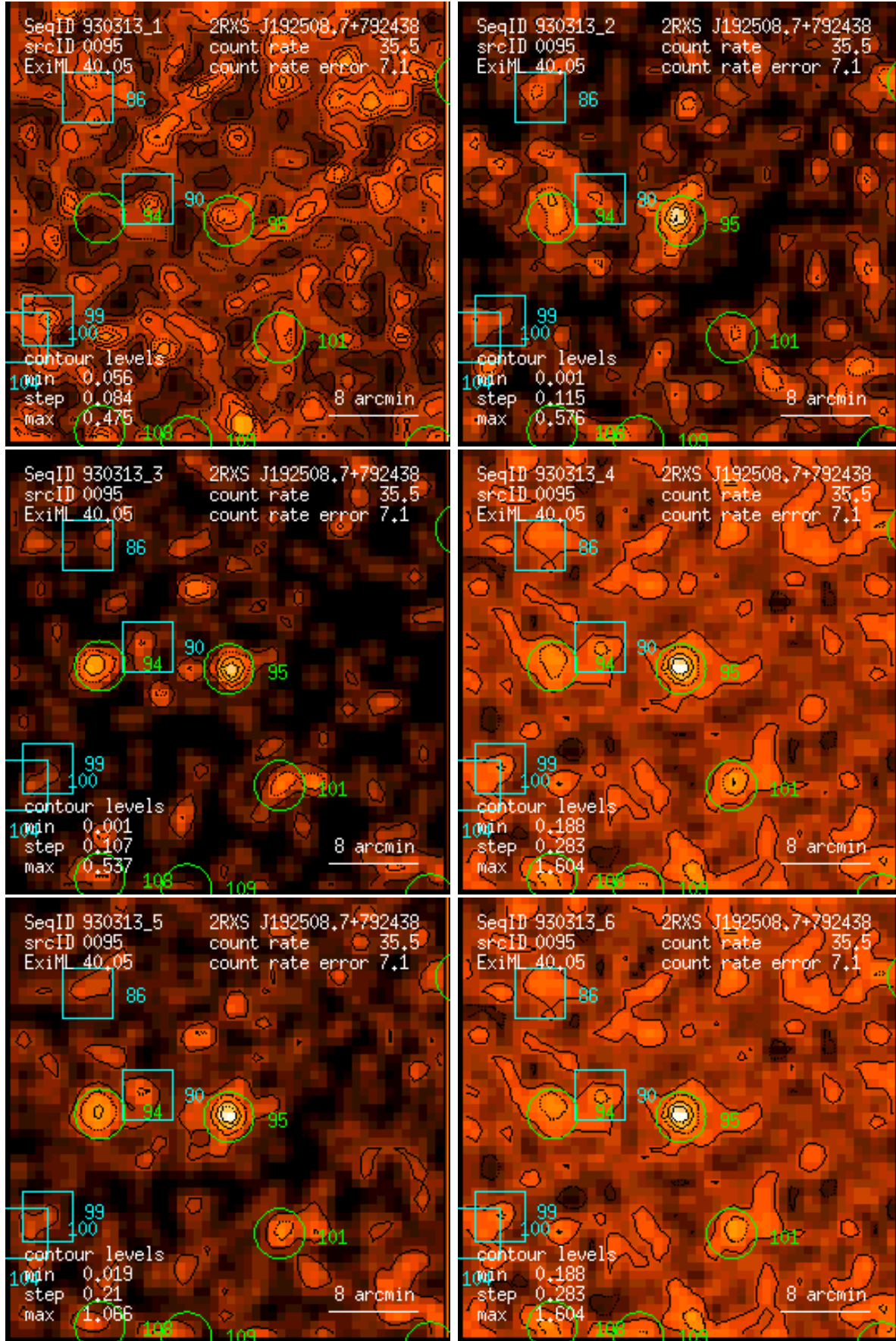
Figure 95: RASS 930313: detection 0095: band rate images, Gaussian filter: (1) PSPC channels 11 – 41, (2) 52 – 90, (3) 91 – 201, (4) 11 – 235, (5) 52 – 201, (6) 11 – 201. Broad band rates in counts/ks. Band rate contour levels in counts/ks/arcmin 2 .
