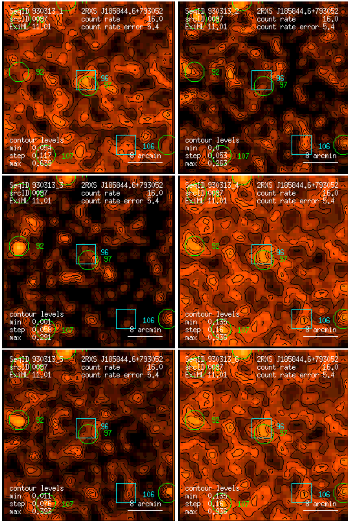
Figure 97: RASS 930313: detection 0097: band rate images, Gaussian filter: (1) PSPC channels 11 – 41, (2) 52 – 90, (3) 91 – 201, (4) 11 – 235, (5) 52 – 201, (6) 11 – 201. Broad band rates in counts/ks. Band rate contour levels in counts/ks/arcmin 2 .
