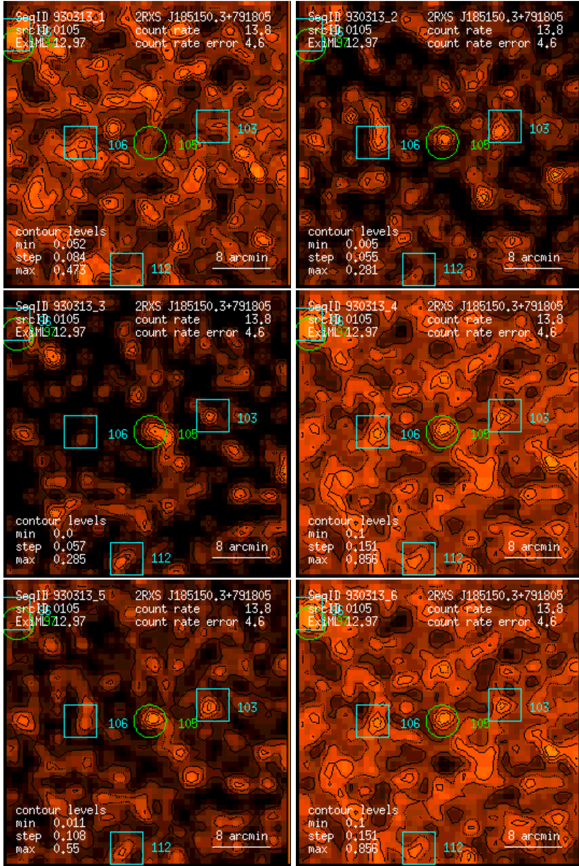
Figure 105: RASS 930313: detection 0105: band rate images, Gaussian filter: (1) PSPC channels 11 – 41, (2) 52 – 90, (3) 91 – 201, (4) 11 – 235, (5) 52 – 201, (6) 11 – 201. Broad band rates in counts/ks. Band rate contour levels in counts/ks/arcmin 2 .
