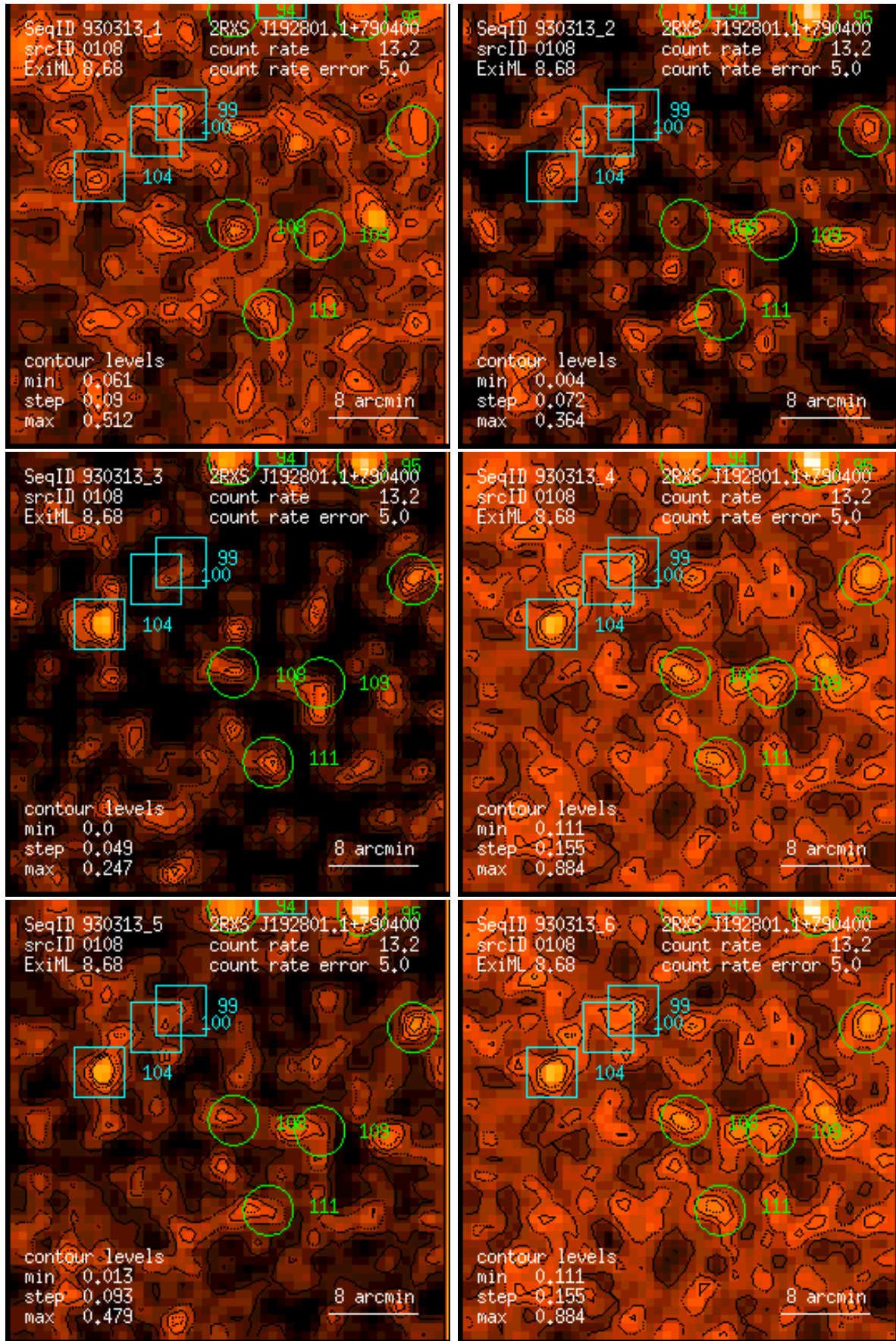
Figure 108: RASS 930313: detection 0108: band rate images, Gaussian filter: (1) PSPC channels 11 – 41, (2) 52 – 90, (3) 91 – 201, (4) 11 – 235, (5) 52 – 201, (6) 11 – 201. Broad band rates in counts/ks. Band rate contour levels in counts/ks/arcmin 2 .
