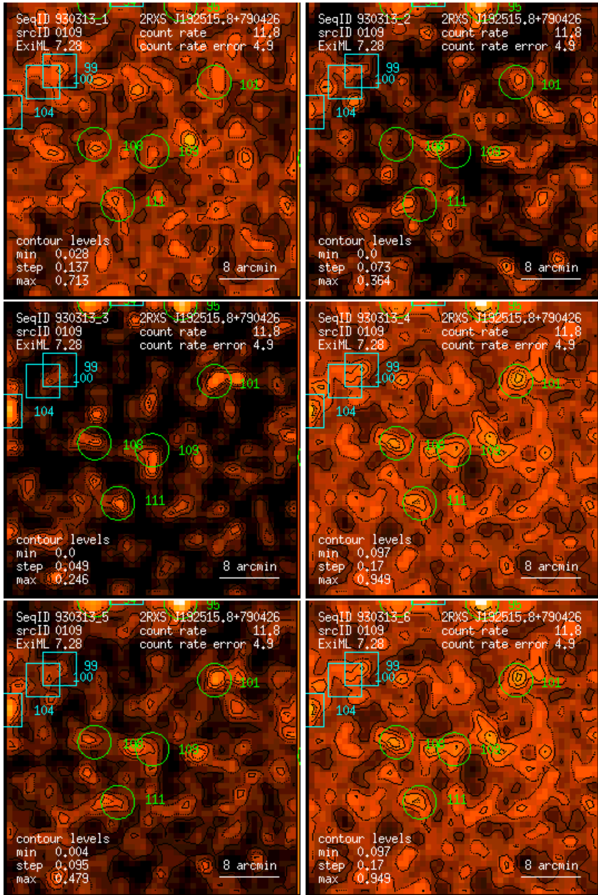
Figure 109: RASS 930313: detection 0109: band rate images, Gaussian filter: (1) PSPC channels 11 – 41, (2) 52 – 90, (3) 91 – 201, (4) 11 – 235, (5) 52 – 201, (6) 11 – 201. Broad band rates in counts/ks. Band rate contour levels in counts/ks/arcmin 2 .
