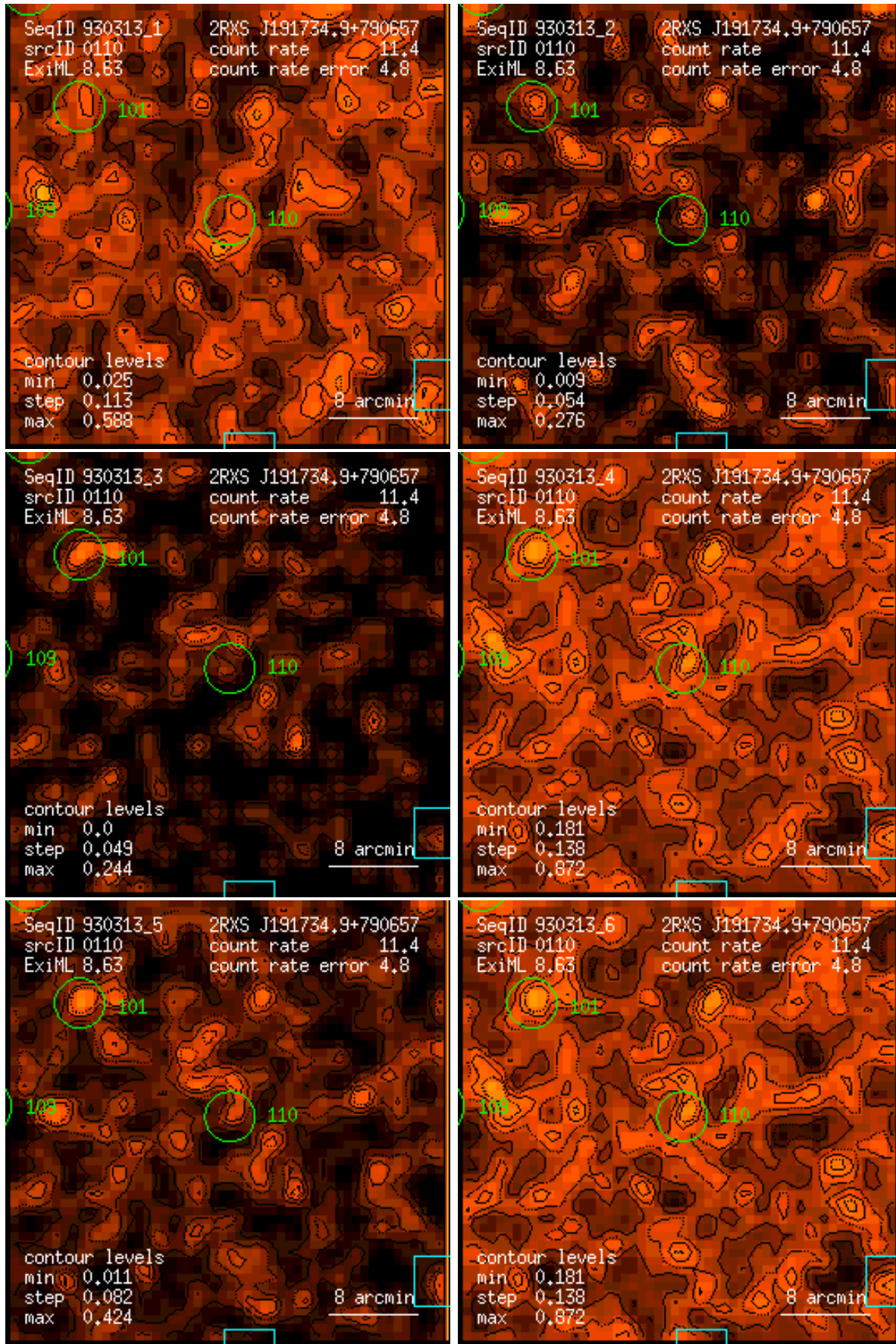
Figure 110: RASS 930313: detection 0110: band rate images, Gaussian filter: (1) PSPC channels 11 – 41, (2) 52 – 90, (3) 91 – 201, (4) 11 – 235, (5) 52 – 201, (6) 11 – 201. Broad band rates in counts/ks. Band rate contour levels in counts/ks/arcmin 2 .
