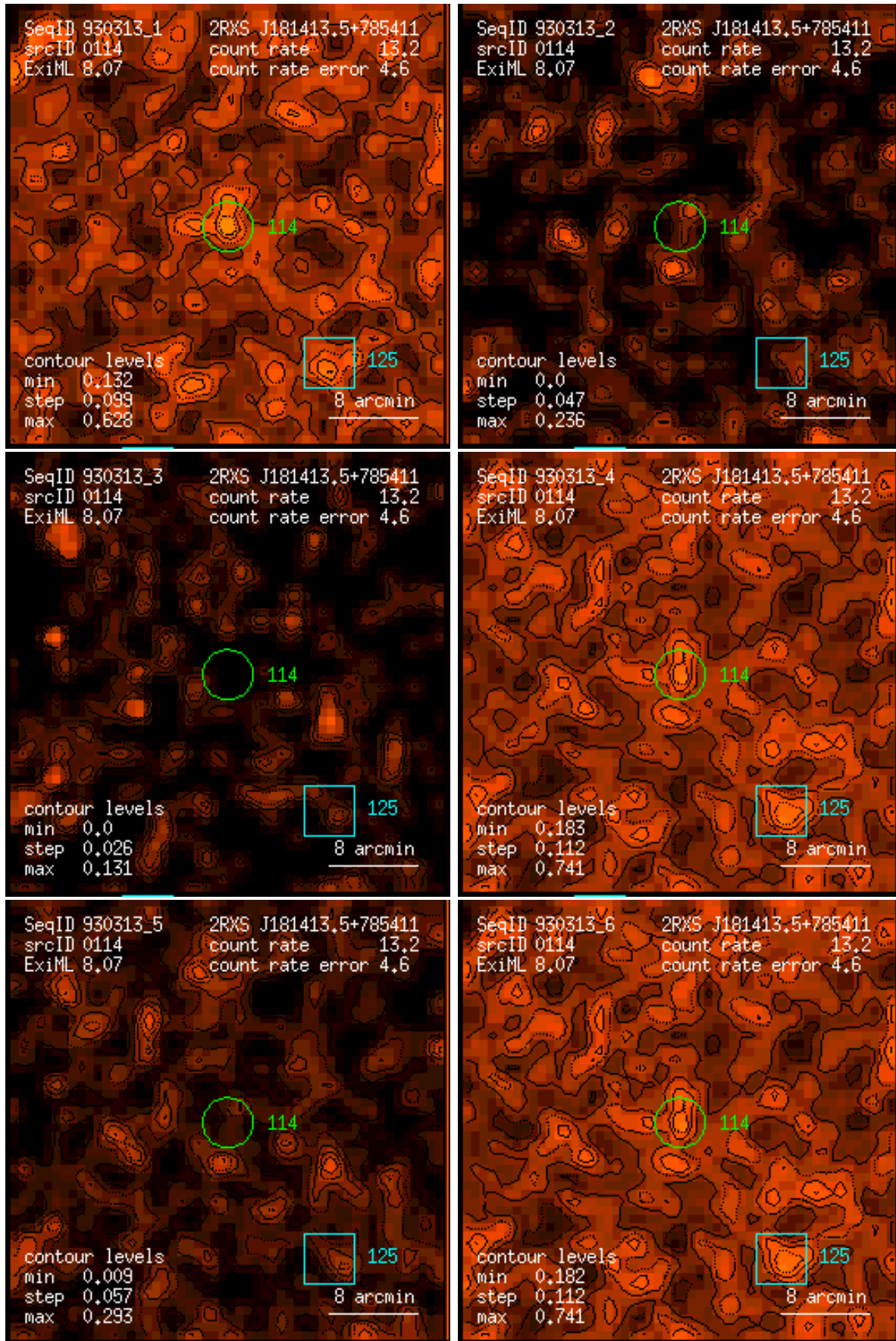
Figure 114: RASS 930313: detection 0114: band rate images, Gaussian filter: (1) PSPC channels 11 – 41, (2) 52 – 90, (3) 91 – 201, (4) 11 – 235, (5) 52 – 201, (6) 11 – 201. Broad band rates in counts/ks. Band rate contour levels in counts/ks/arcmin 2 .
