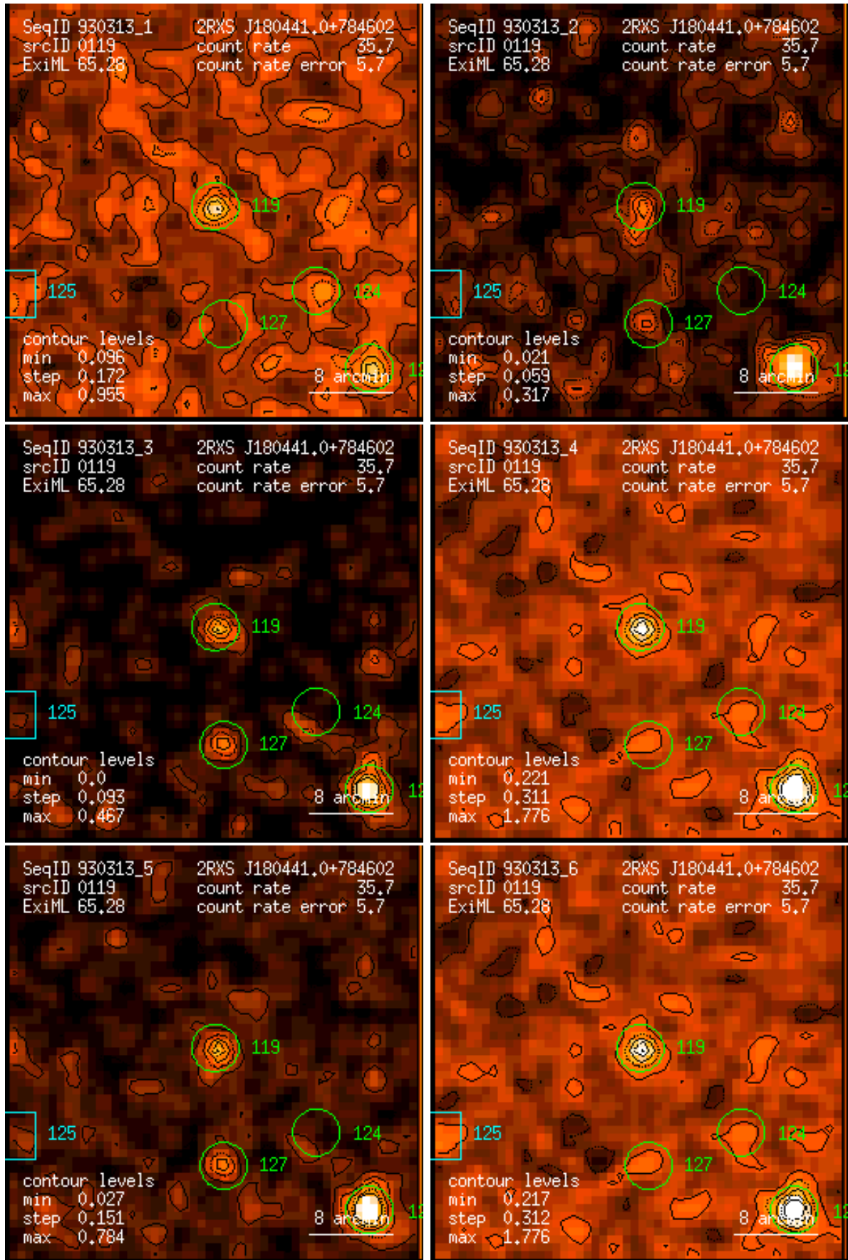
Figure 119: RASS 930313: detection 0119: band rate images, Gaussian filter: (1) PSPC channels 11 – 41, (2) 52 – 90, (3) 91 – 201, (4) 11 – 235, (5) 52 – 201, (6) 11 – 201. Broad band rates in counts/ks. Band rate contour levels in counts/ks/arcmin 2 .
