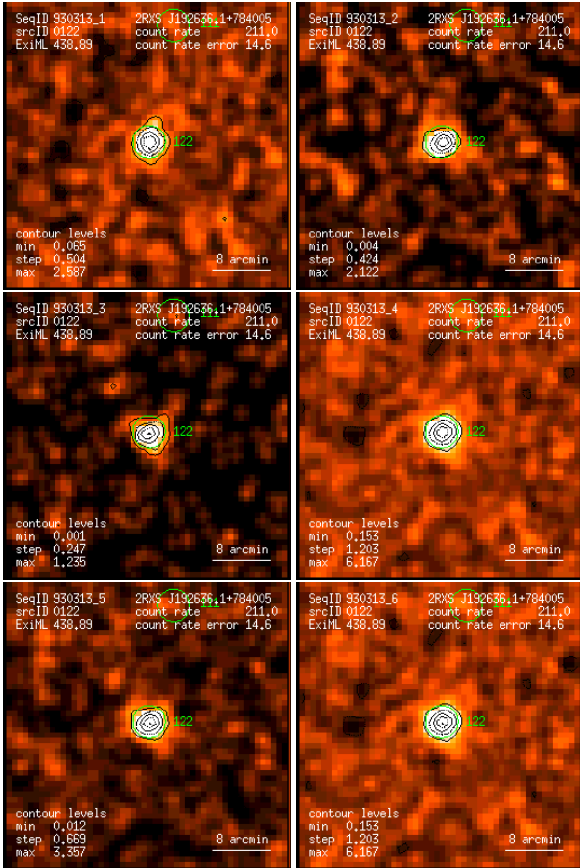
Figure 122: RASS 930313: detection 0122: band rate images, Gaussian filter: (1) PSPC channels 11 – 41, (2) 52 – 90, (3) 91 – 201, (4) 11 – 235, (5) 52 – 201, (6) 11 – 201. Broad band rates in counts/ks. Band rate contour levels in counts/ks/arcmin 2 .
