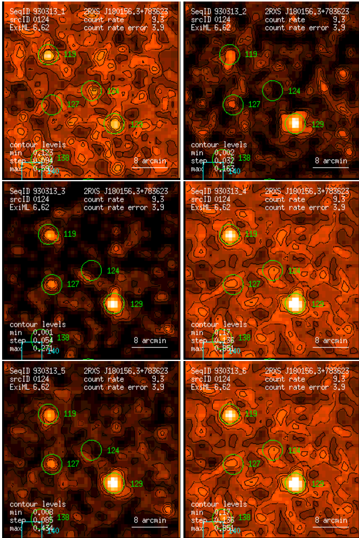
Figure 124: RASS 930313: detection 0124: band rate images, Gaussian filter: (1) PSPC channels 11 – 41, (2) 52 – 90, (3) 91 – 201, (4) 11 – 235, (5) 52 – 201, (6) 11 – 201. Broad band rates in counts/ks. Band rate contour levels in counts/ks/arcmin 2 .
