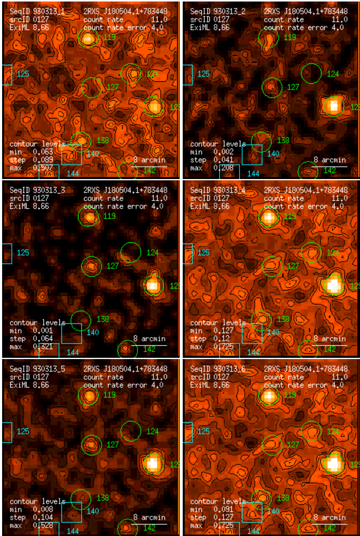
Figure 127: RASS 930313: detection 0127: band rate images, Gaussian filter: (1) PSPC channels 11 – 41, (2) 52 – 90, (3) 91 – 201, (4) 11 – 235, (5) 52 – 201, (6) 11 – 201. Broad band rates in counts/ks. Band rate contour levels in counts/ks/arcmin 2 .
