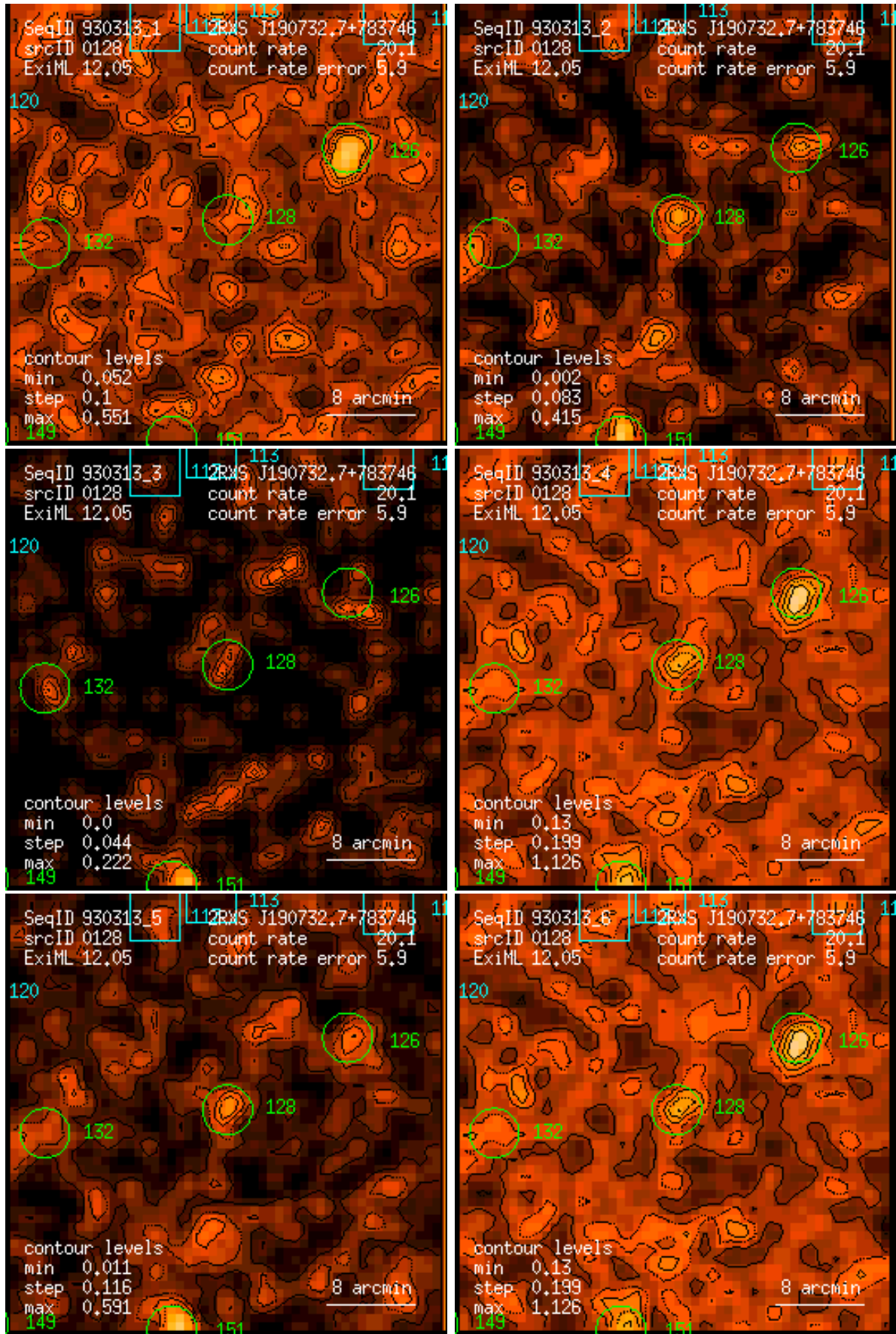
Figure 128: RASS 930313: detection 0128: band rate images, Gaussian filter: (1) PSPC channels 11 – 41, (2) 52 – 90, (3) 91 – 201, (4) 11 – 235, (5) 52 – 201, (6) 11 – 201. Broad band rates in counts/ks. Band rate contour levels in counts/ks/arcmin 2 .
