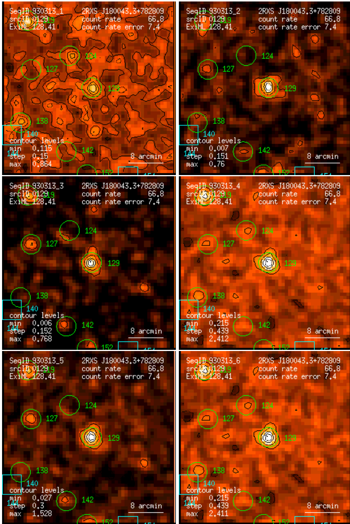
Figure 129: RASS 930313: detection 0129: band rate images, Gaussian filter: (1) PSPC channels 11 – 41, (2) 52 – 90, (3) 91 – 201, (4) 11 – 235, (5) 52 – 201, (6) 11 – 201. Broad band rates in counts/ks. Band rate contour levels in counts/ks/arcmin 2 .
