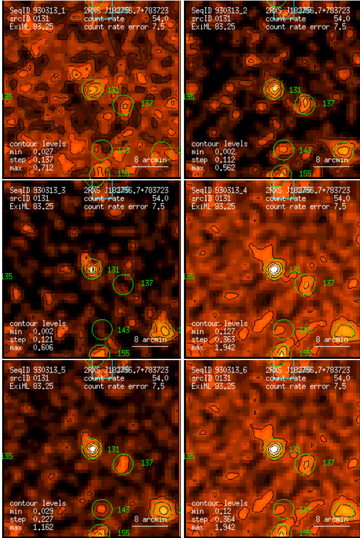
Figure 131: RASS 930313: detection 0131: band rate images, Gaussian filter: (1) PSPC channels 11 – 41, (2) 52 – 90, (3) 91 – 201, (4) 11 – 235, (5) 52 – 201, (6) 11 – 201. Broad band rates in counts/ks. Band rate contour levels in counts/ks/arcmin 2 .
