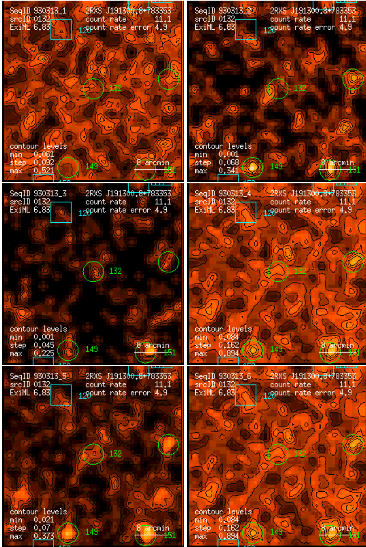
Figure 132: RASS 930313: detection 0132: band rate images, Gaussian filter: (1) PSPC channels 11 – 41, (2) 52 – 90, (3) 91 – 201, (4) 11 – 235, (5) 52 – 201, (6) 11 – 201. Broad band rates in counts/ks. Band rate contour levels in counts/ks/arcmin 2 .
