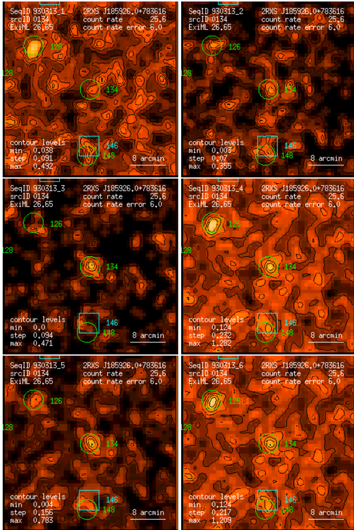
Figure 134: RASS 930313: detection 0134: band rate images, Gaussian filter: (1) PSPC channels 11 – 41, (2) 52 – 90, (3) 91 – 201, (4) 11 – 235, (5) 52 – 201, (6) 11 – 201. Broad band rates in counts/ks. Band rate contour levels in counts/ks/arcmin 2 .
